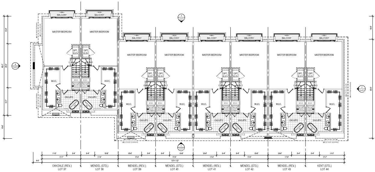
1 THIRD FLOOR SCALE: 1/8" = 1'-0"
