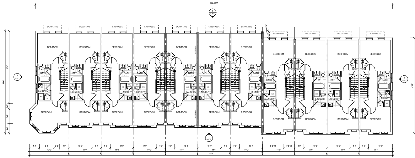
SECOND FLOOR SCALE: 1/8" = 1'-0"
