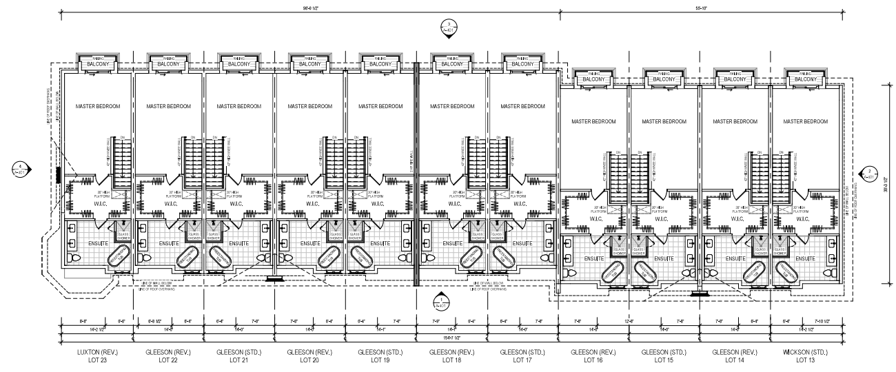
1 A20 THIRD FLOOR SCALE: 1/8" = 1'-0"
