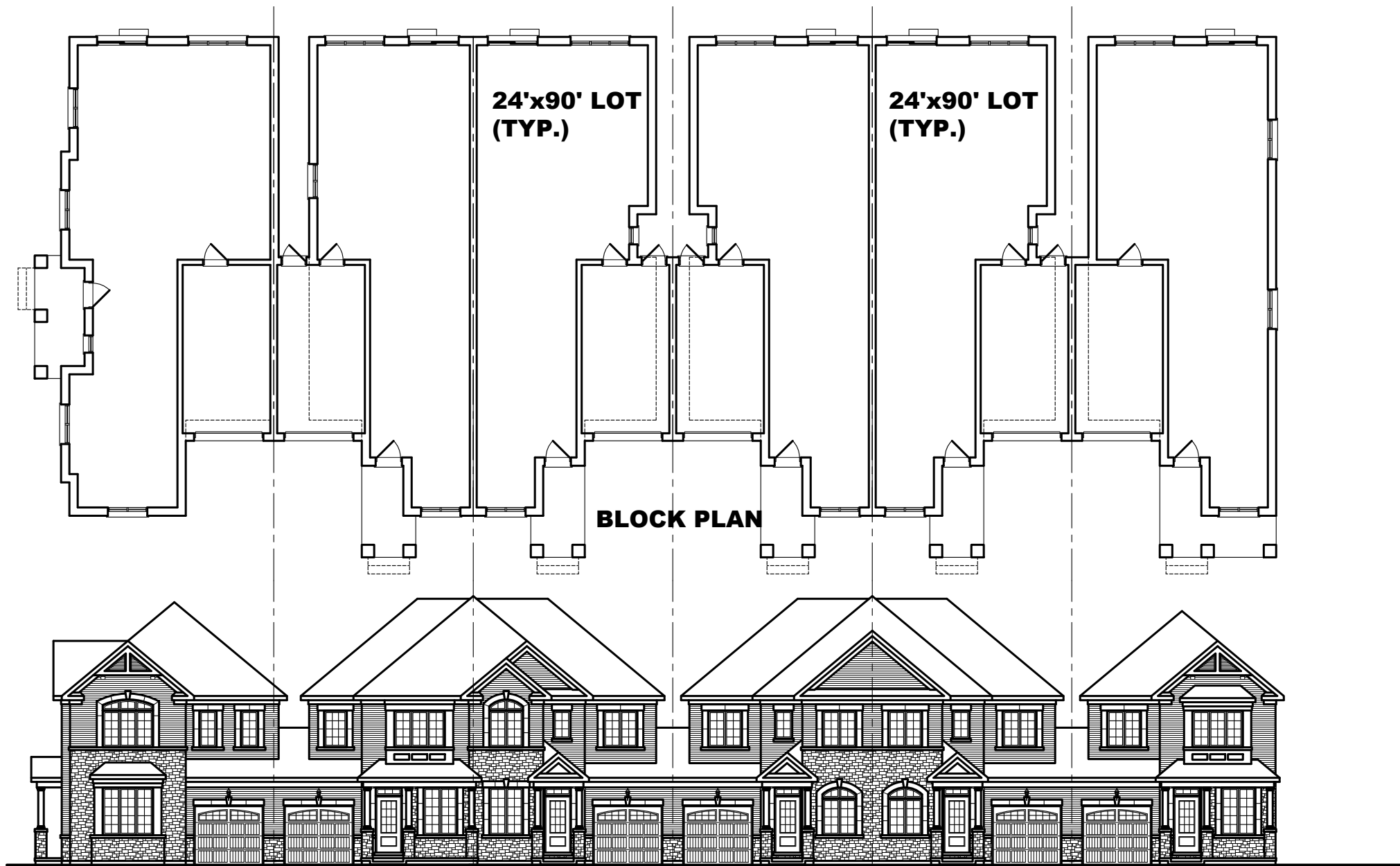
24'x90' SEMI-TOWNHOUSE
