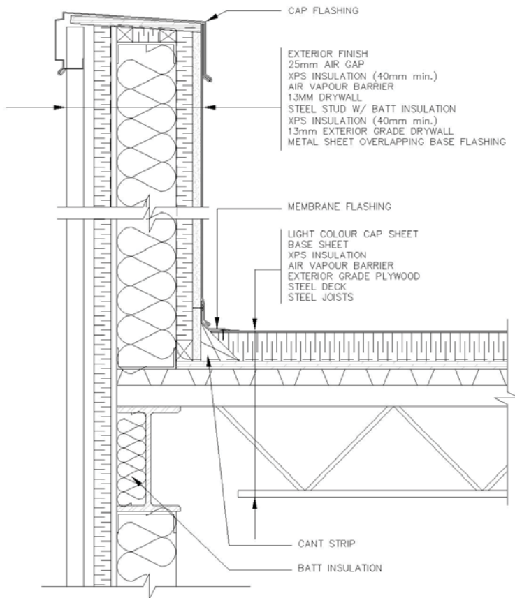
Detail 4 - Parapet
