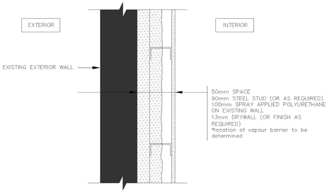
Detail 3 – Interior insulation
