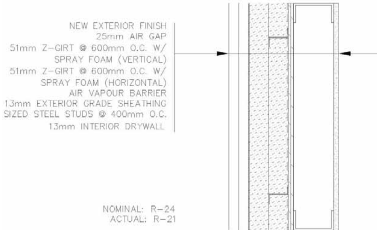
Detail 1 – Continuous Layer of Insulation
