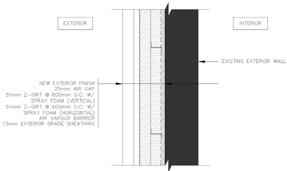
Detail 2 – Exterior insulation
