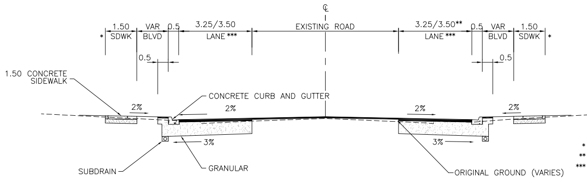
TYPICAL SECTION SPEERS ROAD AND NORTH SERVICE ROAD EAST OF FOURTH LINE
