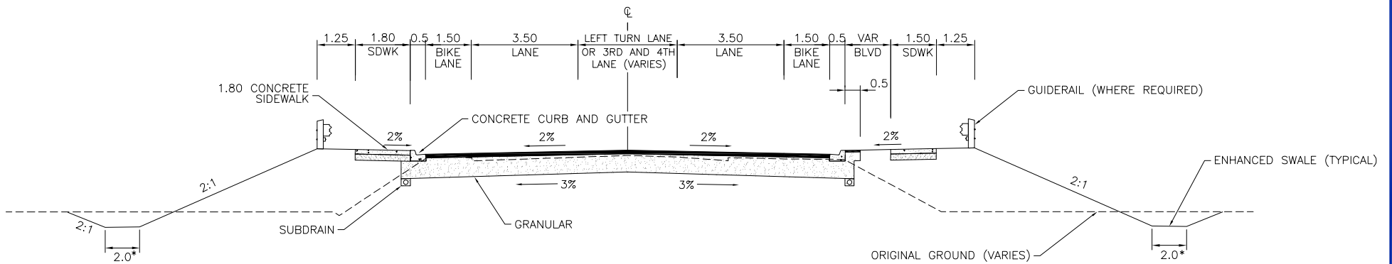
TYPICAL SECTION SOUTH SERVICE ROAD/WYECROFT ROAD NORTH SERVICE ROAD WEST OF FOURTH LINE AND FOURTH LINE
