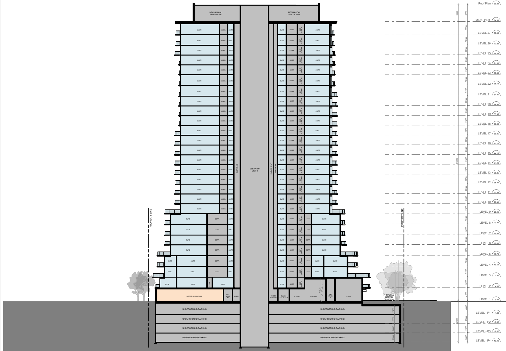
Building Section 'A' 1 : 200
