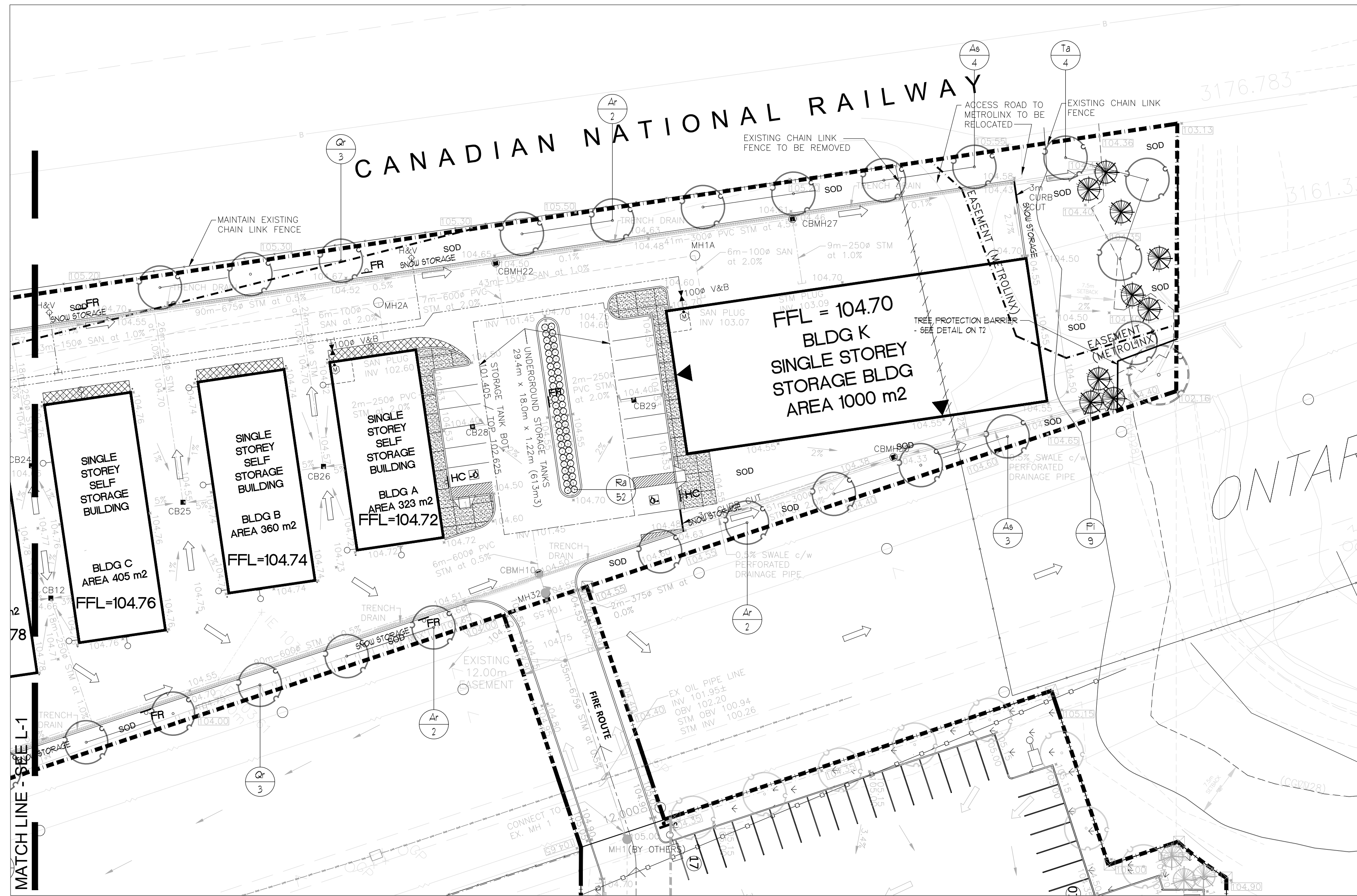
LANDSCAPE PLAN 'B' SCALE = 1:400
