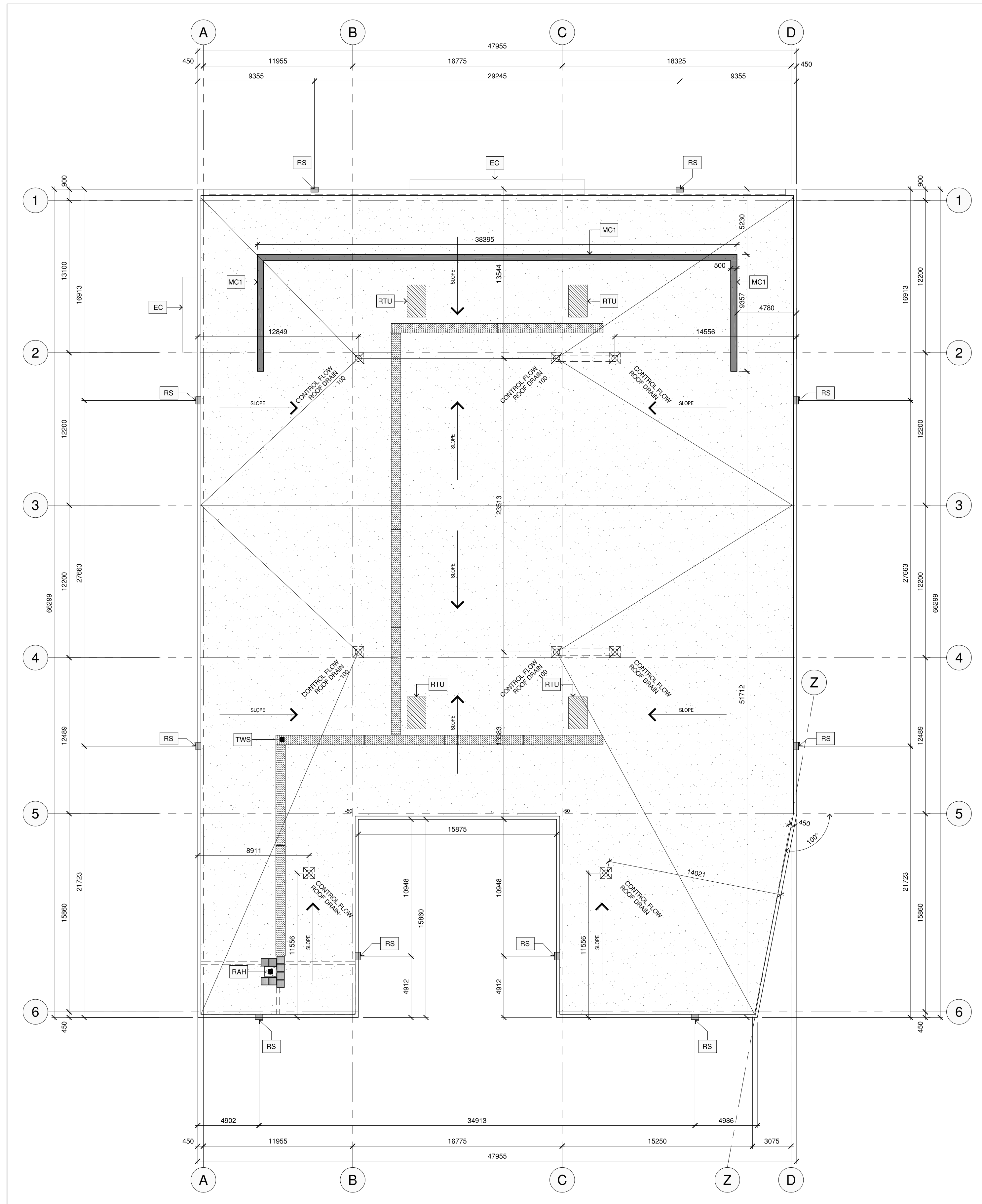
1 ROOF PLAN SCALE 1:200
