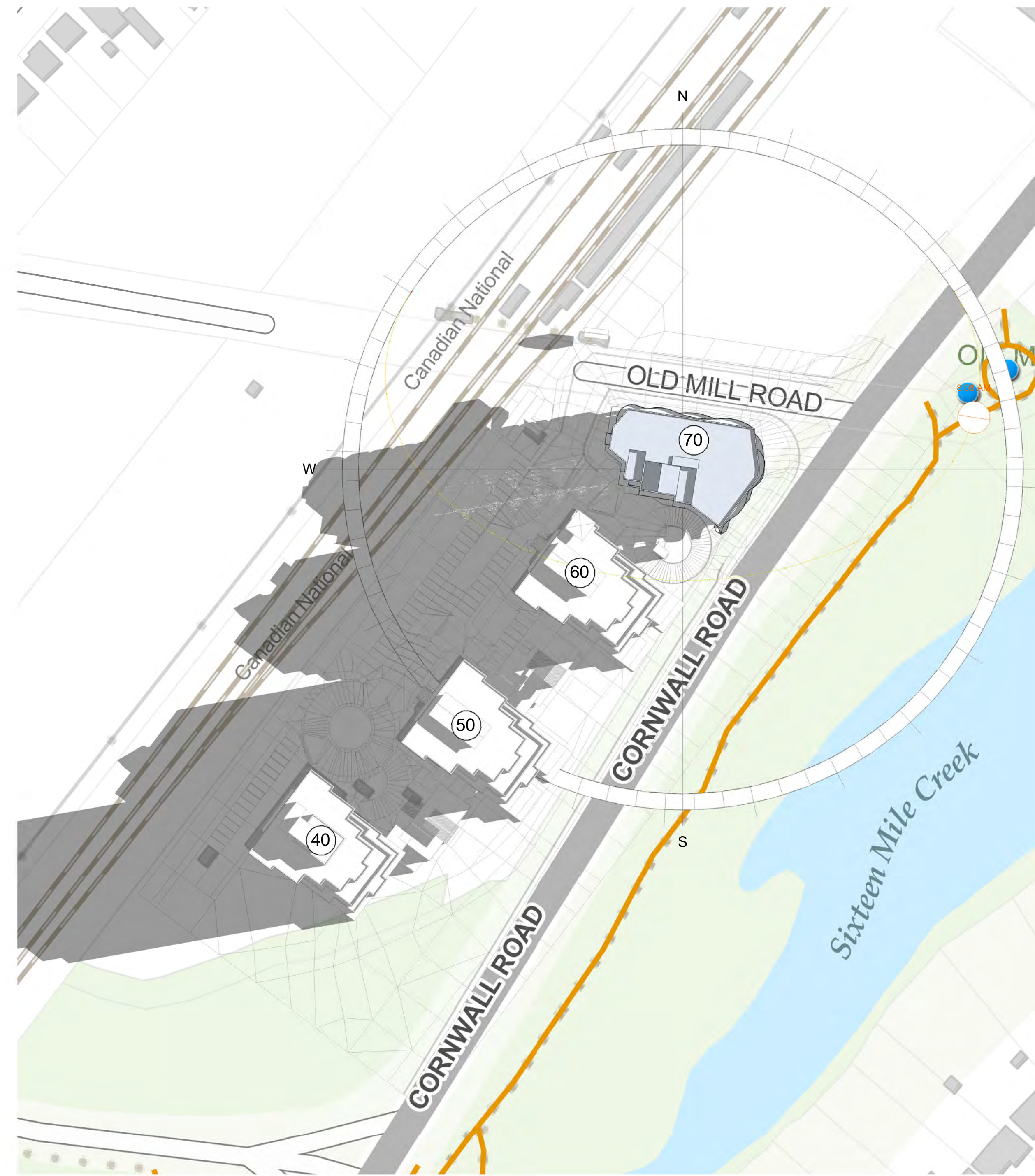
2 SUN & SHADOW STUDY - JUN. 21 - 8.08 a.m. 1 : 1000
