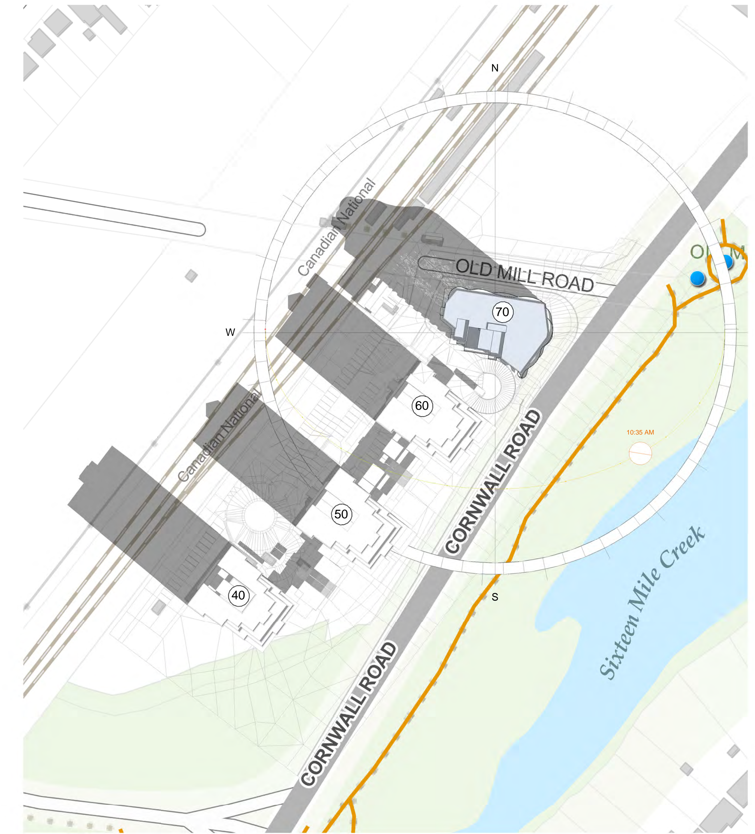
3 SUN & SHADOW STUDY - SEPT. 21 - 10.35 a.m. 1 : 1000
