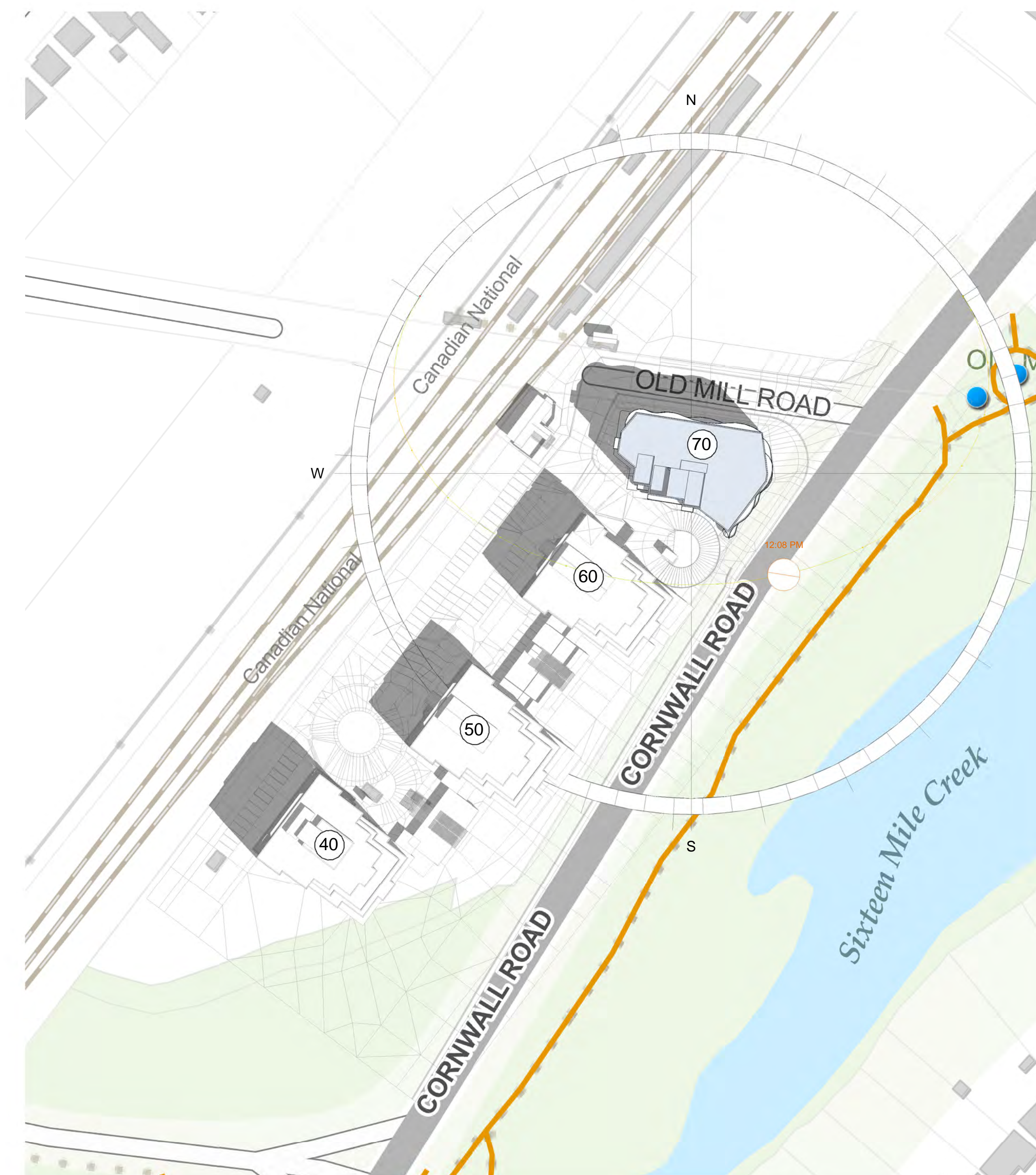
6 SUN & SHADOW STUDY - JUN. 21 - 12.08 p.m. 1 : 1000
