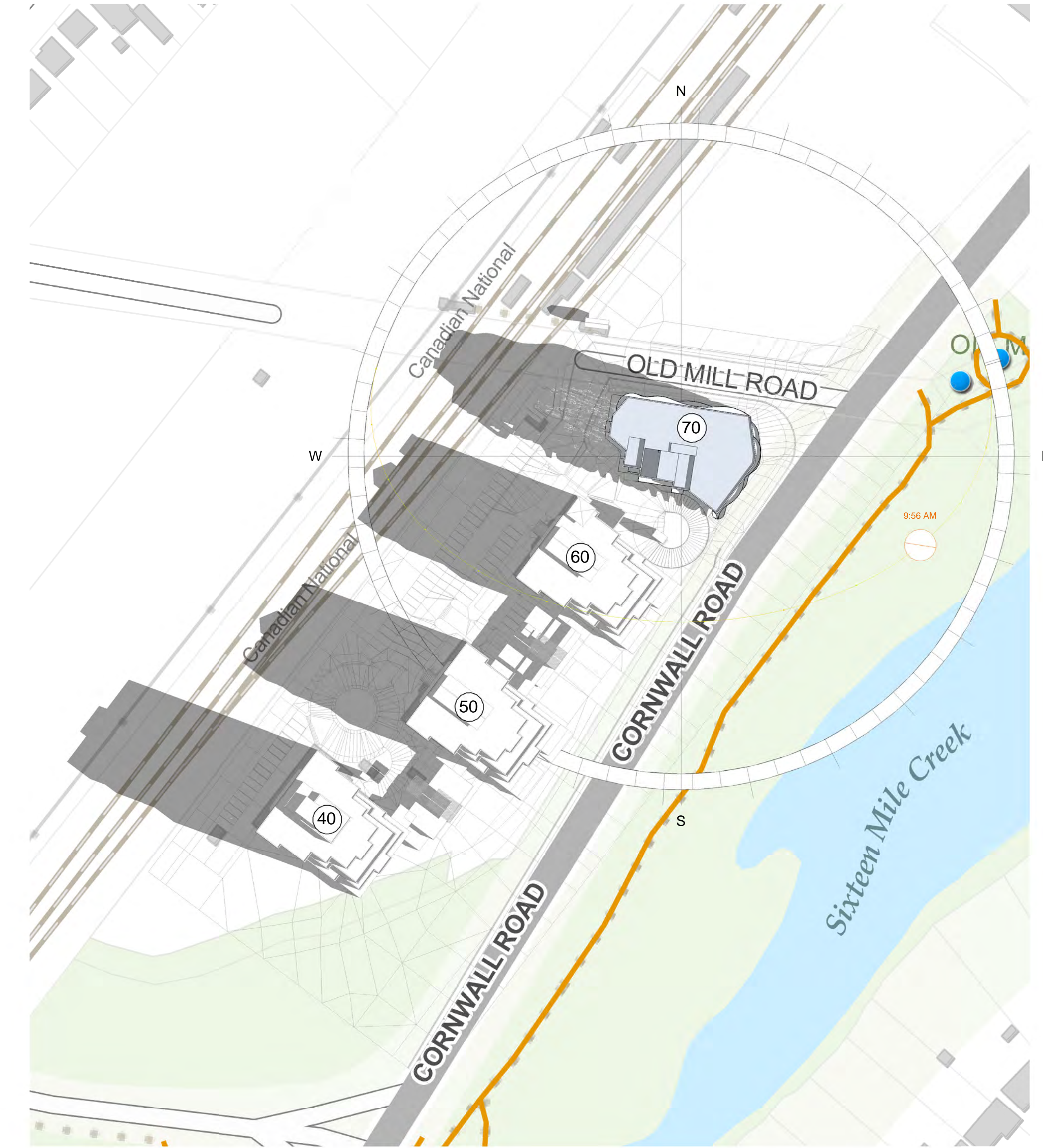
3 SUN & SHADOW STUDY - APR. 21 - 9.56 a.m. 1 : 1000
