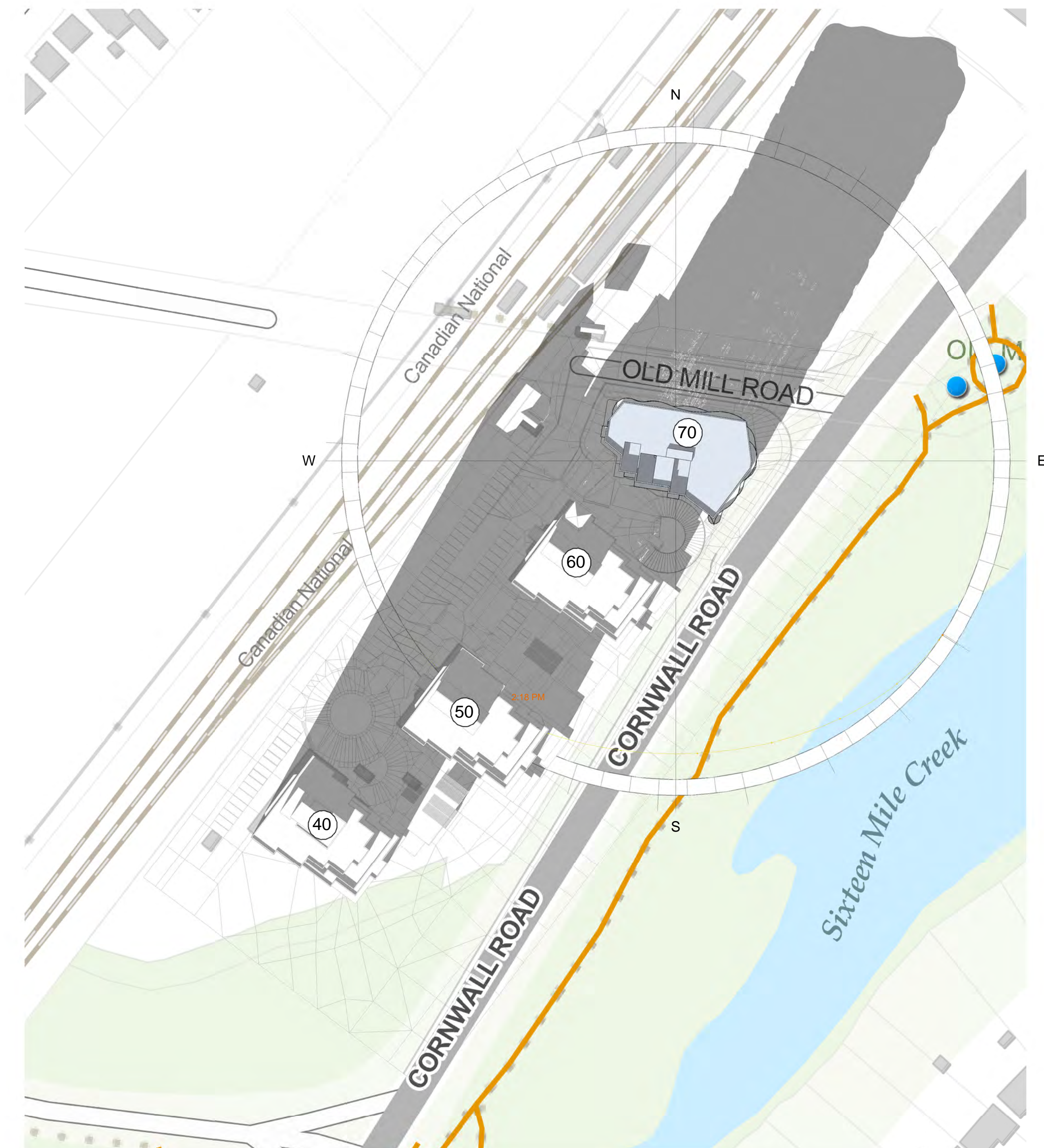
6 SUN & SHADOW STUDY - DEC. 21 - 2.18 p.m. 1 : 1000
