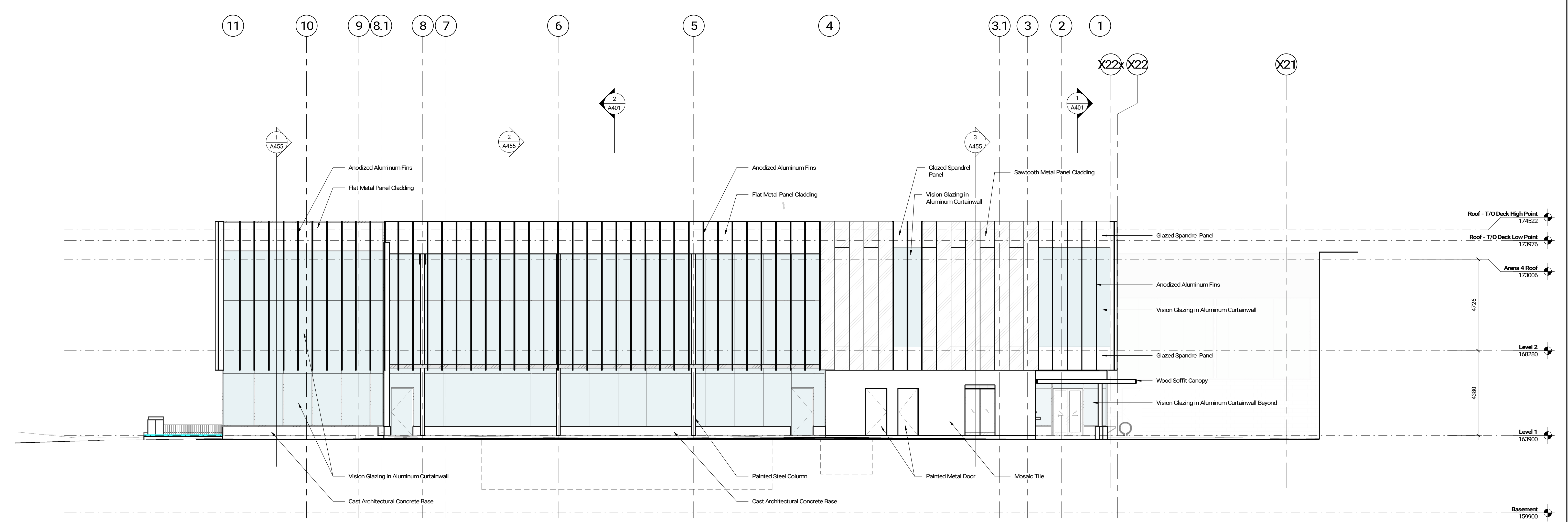
North Elevation 1:100 A301
