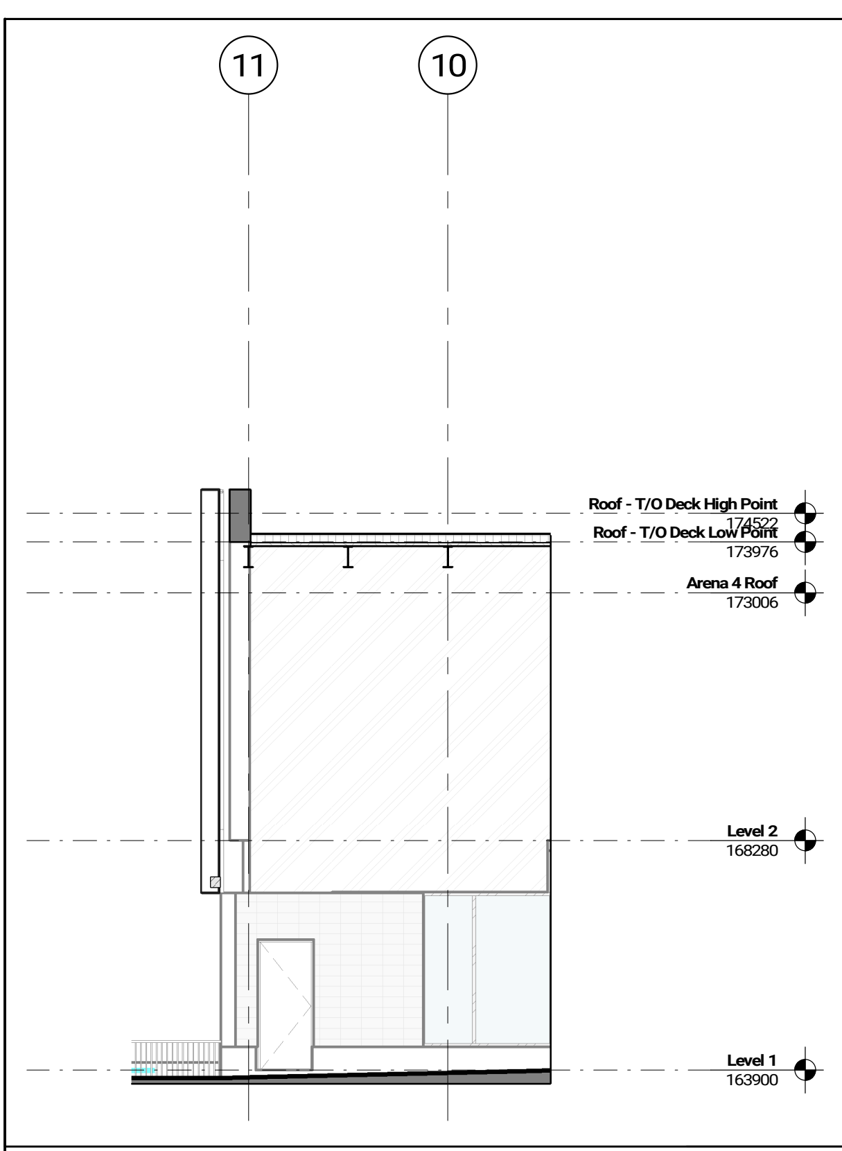
South Elevation - Play Area 1:100 A302
