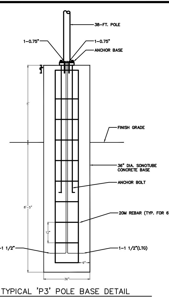
TYPICAL 'P3' POLE BASE DETAIL N.T.S.
