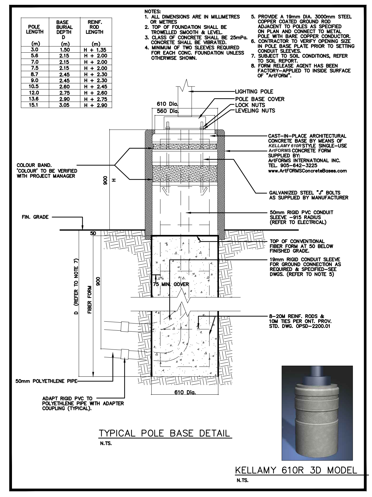
TYPICAL POLE BASE DETAIL N.T.S. KELLAMY 610R 3D MODEL N.T.S.
