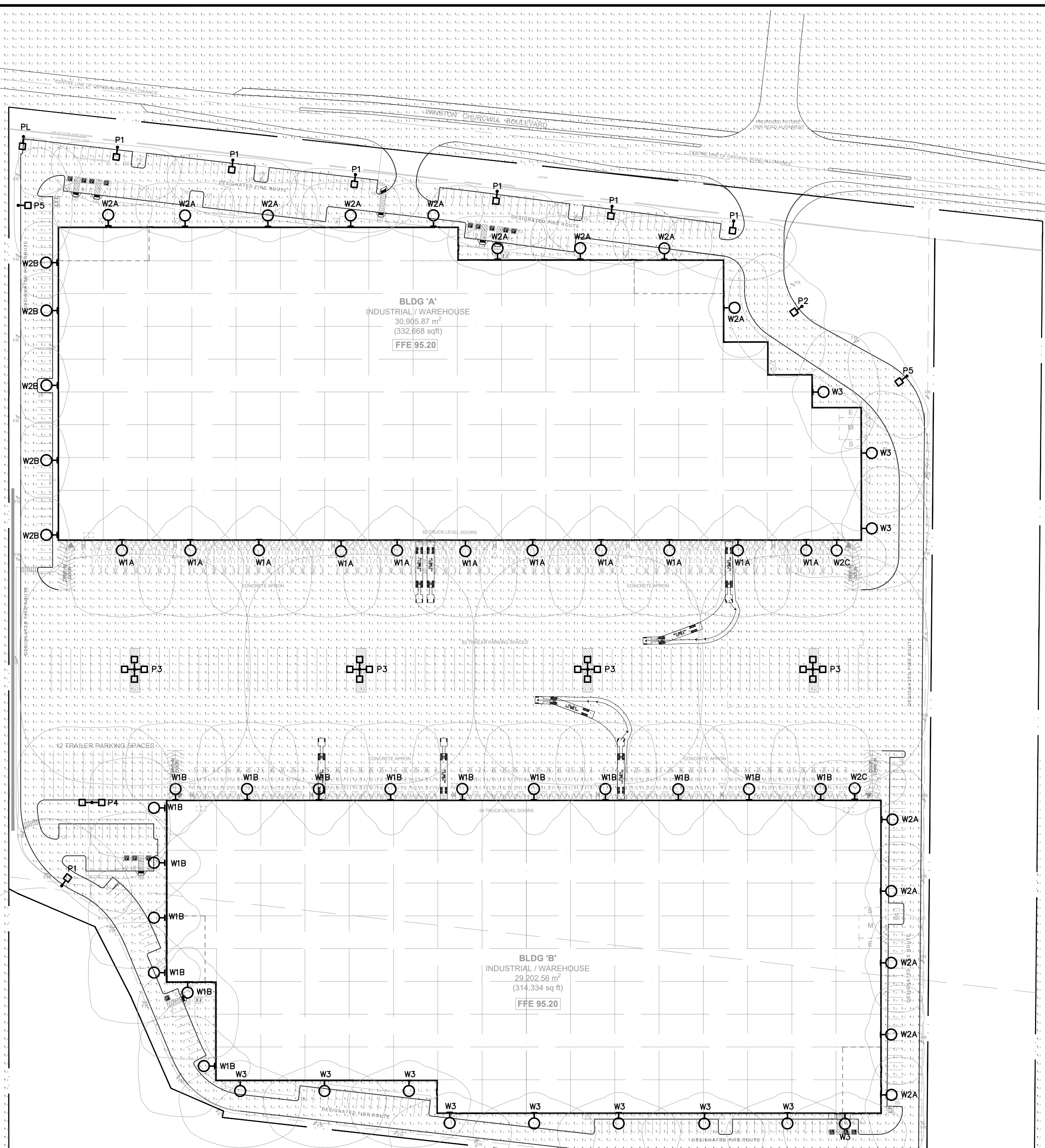
ELECTRICAL SITE PLAN SCALE: 1:1000
