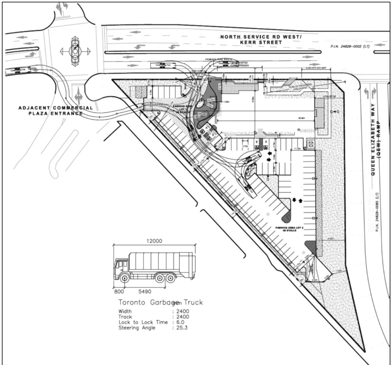
Figure 8-3 AutoTURN Analysis for Garbage Truck Vehicle (Custom)
