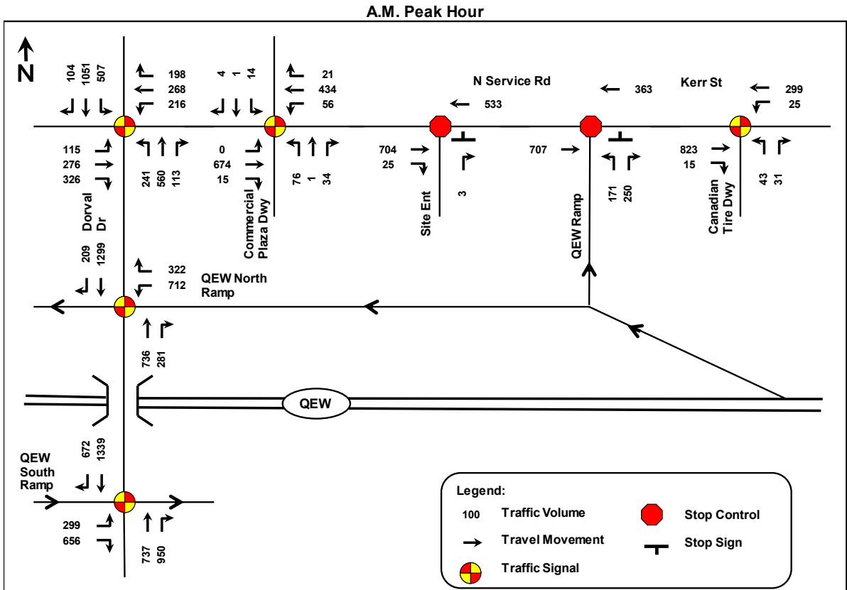
Figure 6-6 Future Total Peak Hour Traffic Volumes – 2028
