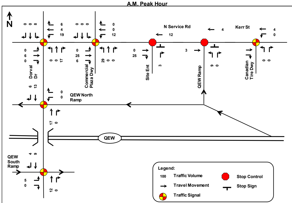
Figure 6-4 Total Peak Hour Proposed Site Development Related Trips
