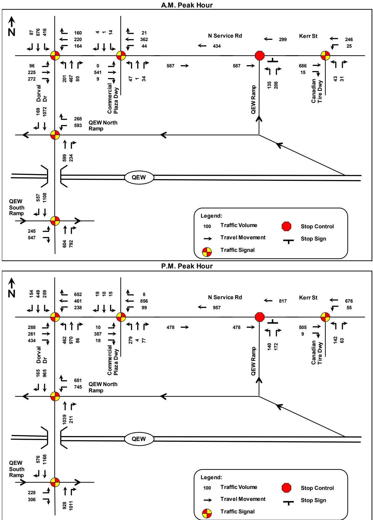
Figure 6-1 Existing Peak Hour Traffic Volumes
