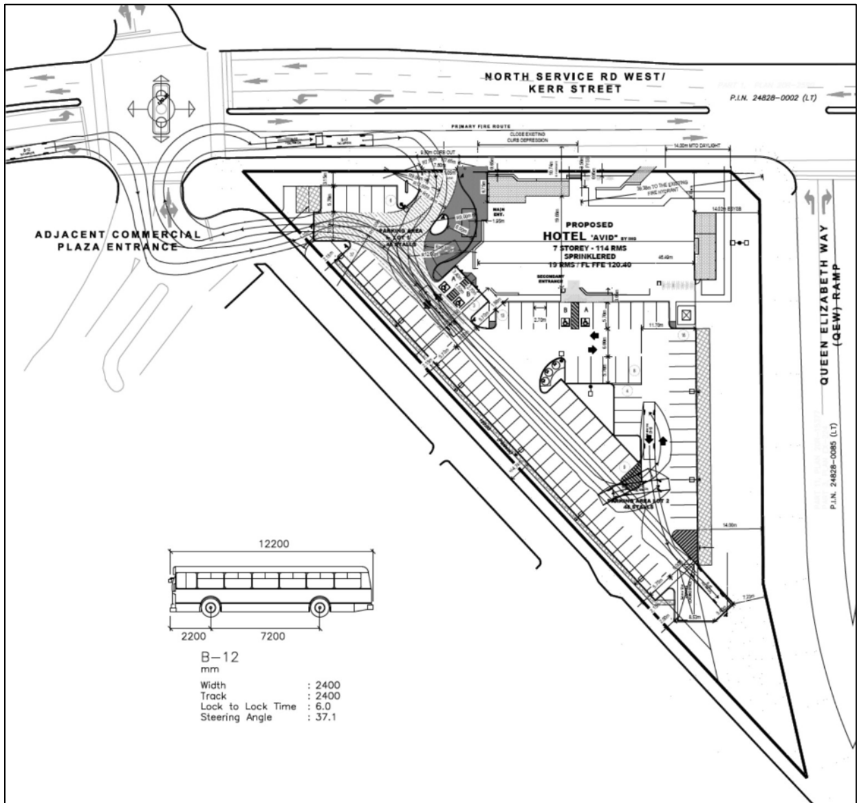
Figure 8-1 AutoTURN Analysis for Bus (TAC-1999 B)
