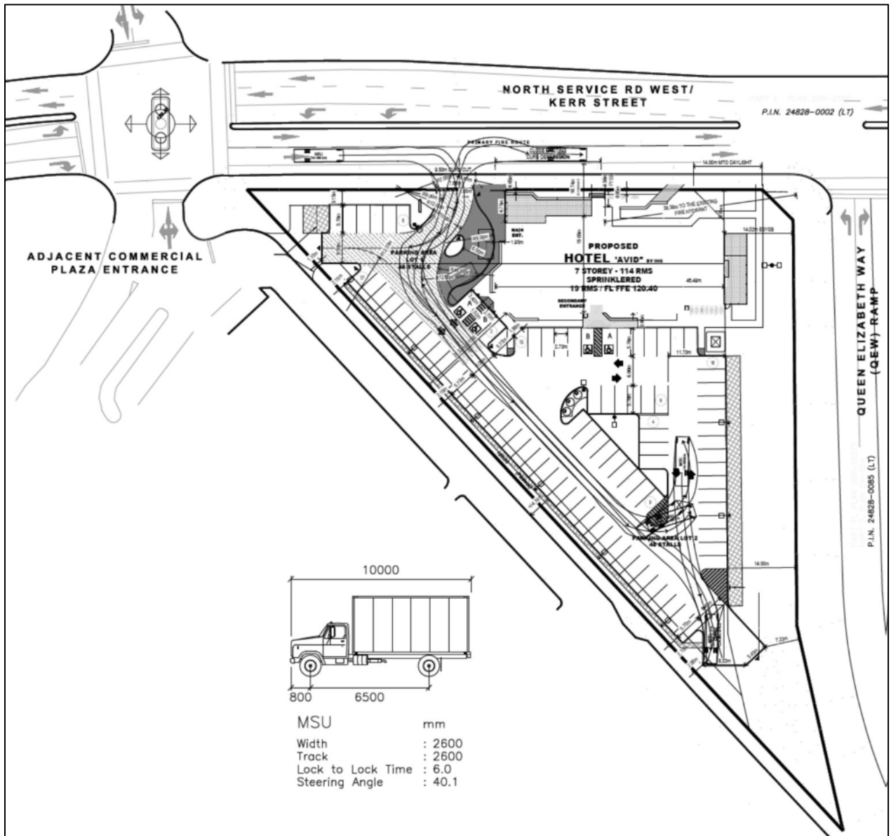
Figure 8-2 AutoTURN Analysis for Medium Single Unit Vehicle (TAC-1999 MSU)
