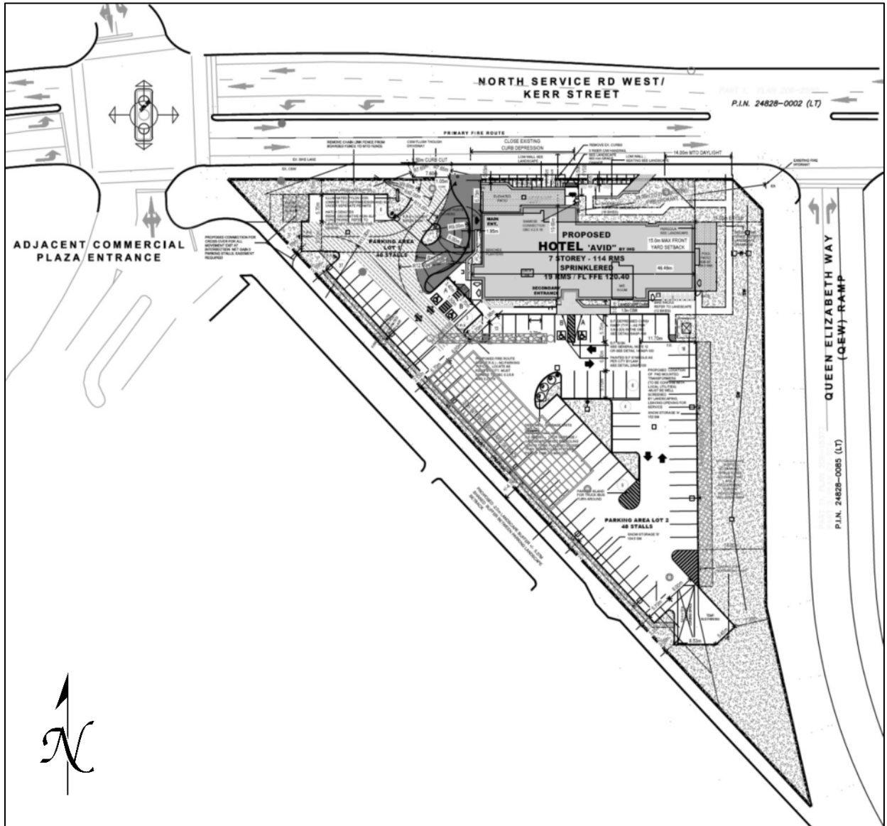
Figure 1-2 Proposed Site Plan
