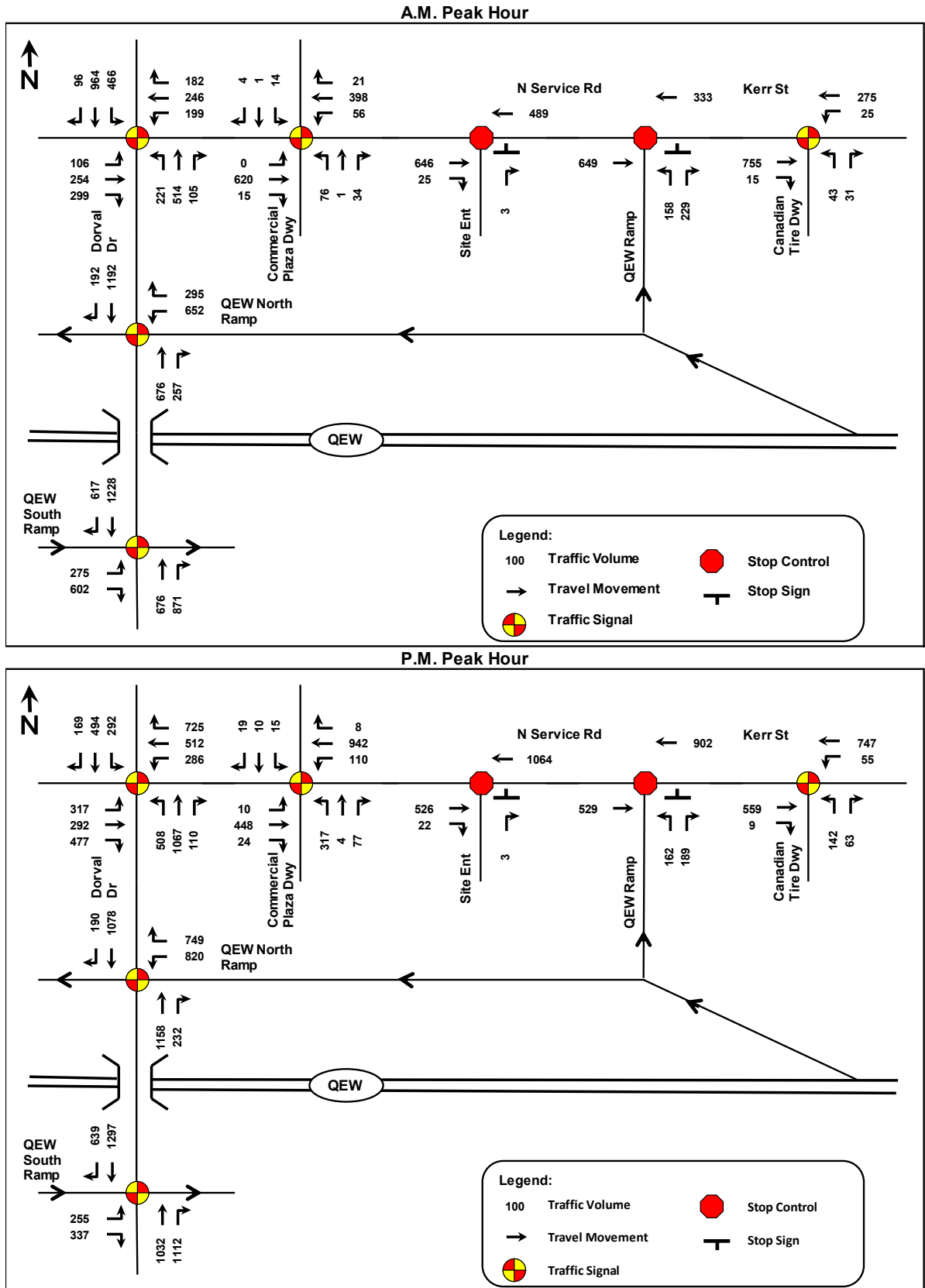
Figure 6-5 Future Total Peak Hour Traffic Volumes – 2023
