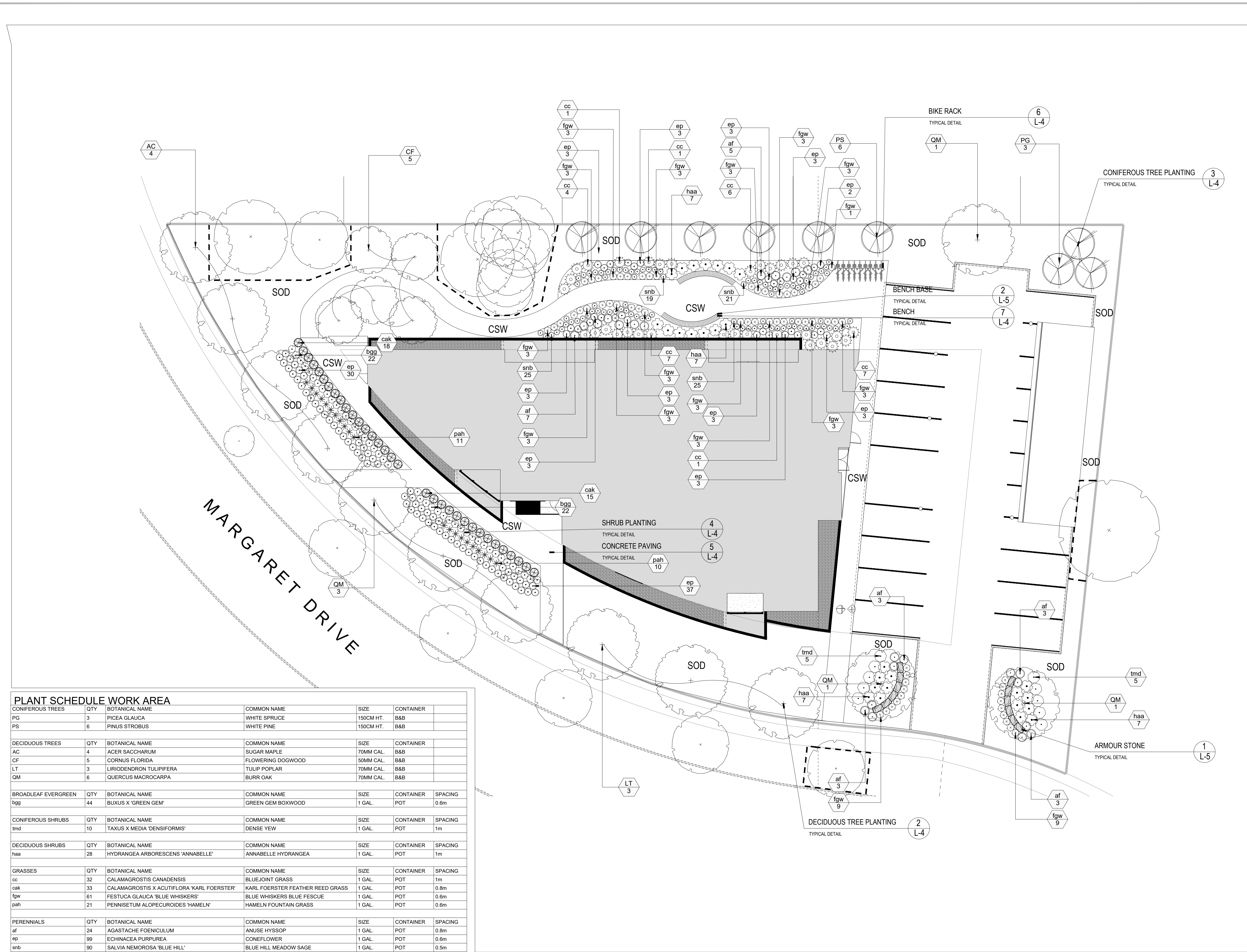
1 LANDSCAPE PLAN L-1 1:150
