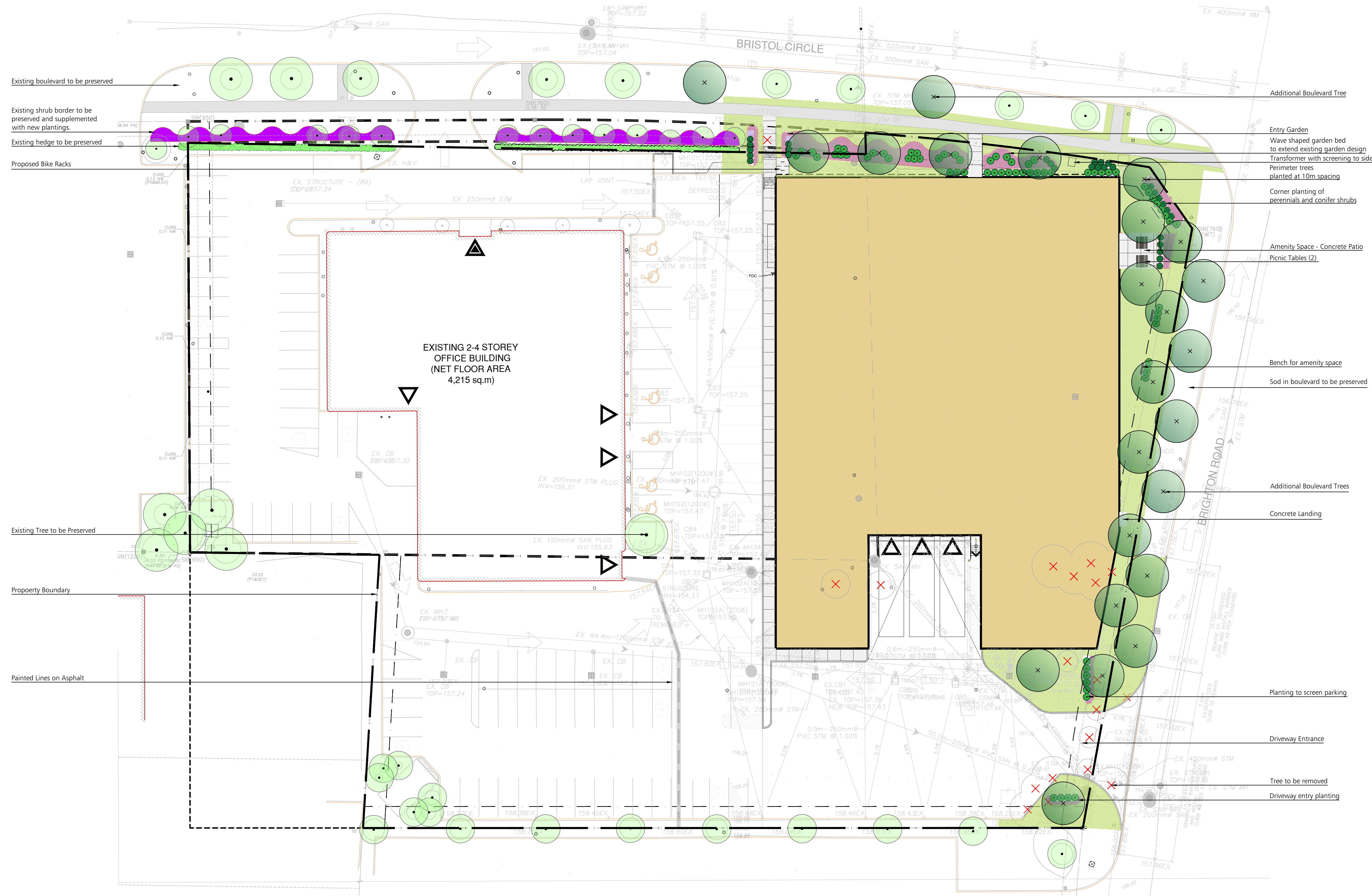
LANDSCAPE CONCEPT PLAN 1:300
