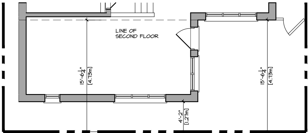
PARTIAL PLAN AT REAR
