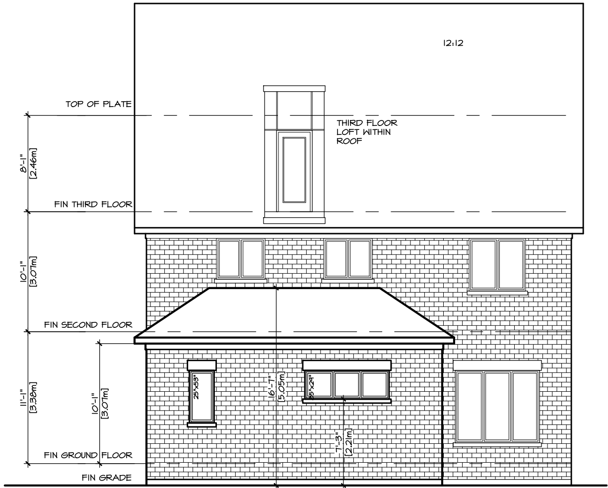
ONE STOREY PROJECTION AT REAR
