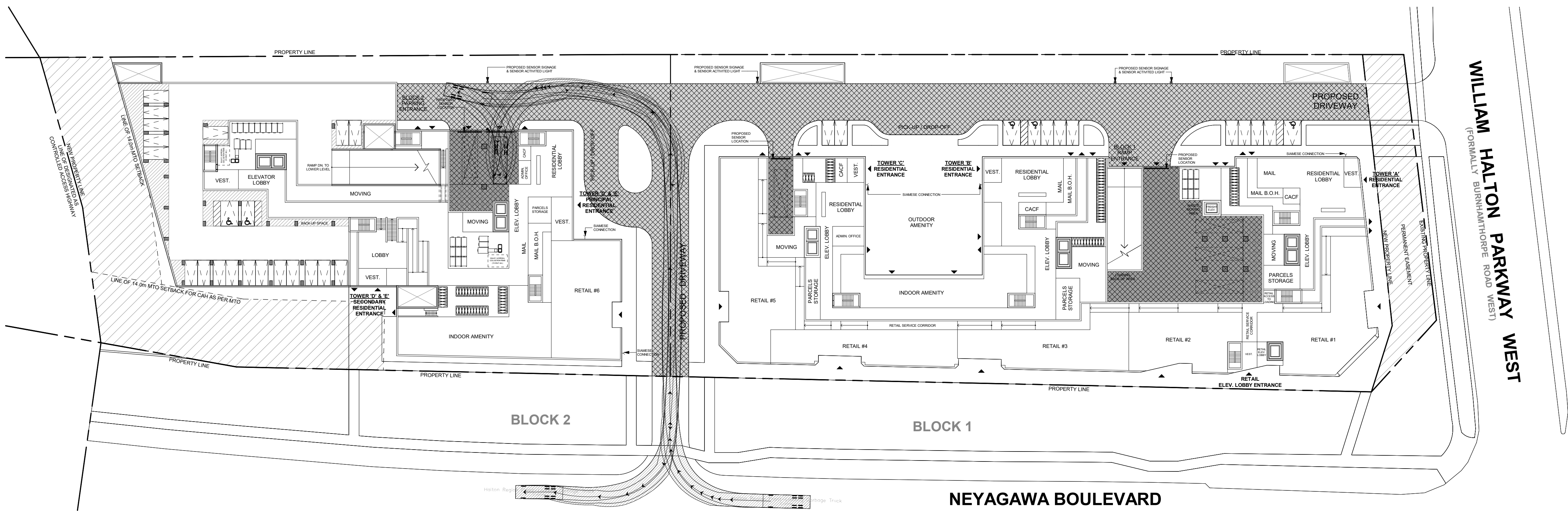
2 Waste Collection Vehicle Movement Diagram - Tower 'D' - Residential
