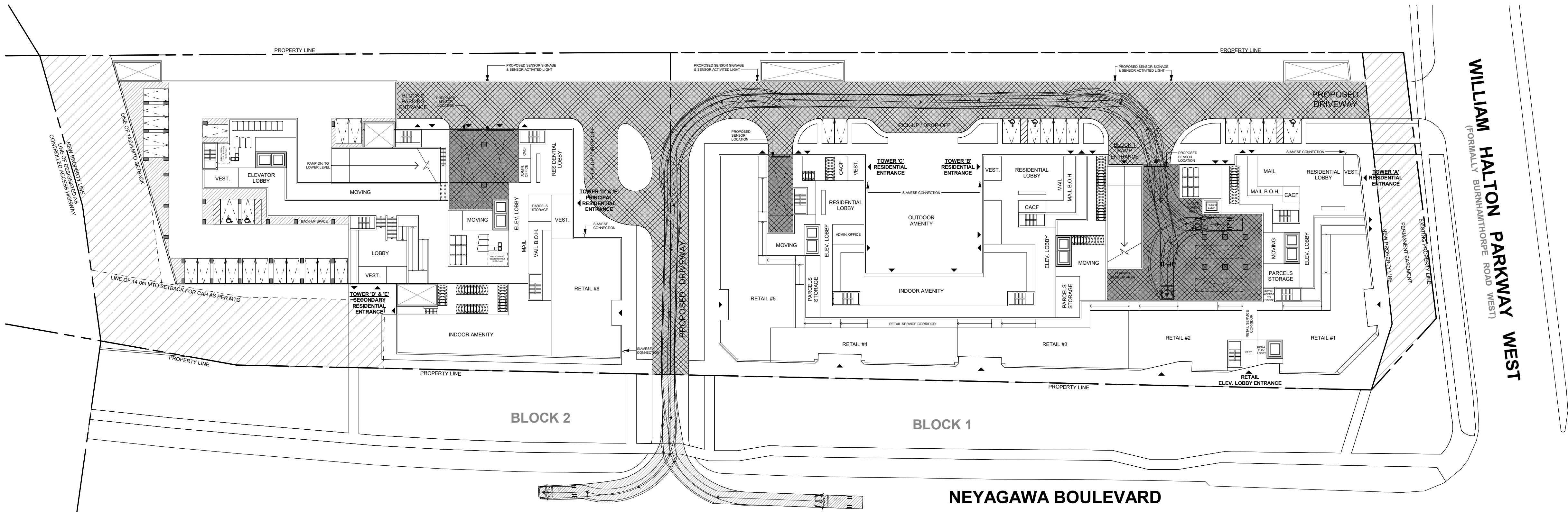
1 Tower 'A' - Retail Waste Collection Vehicle Movement Diagram
