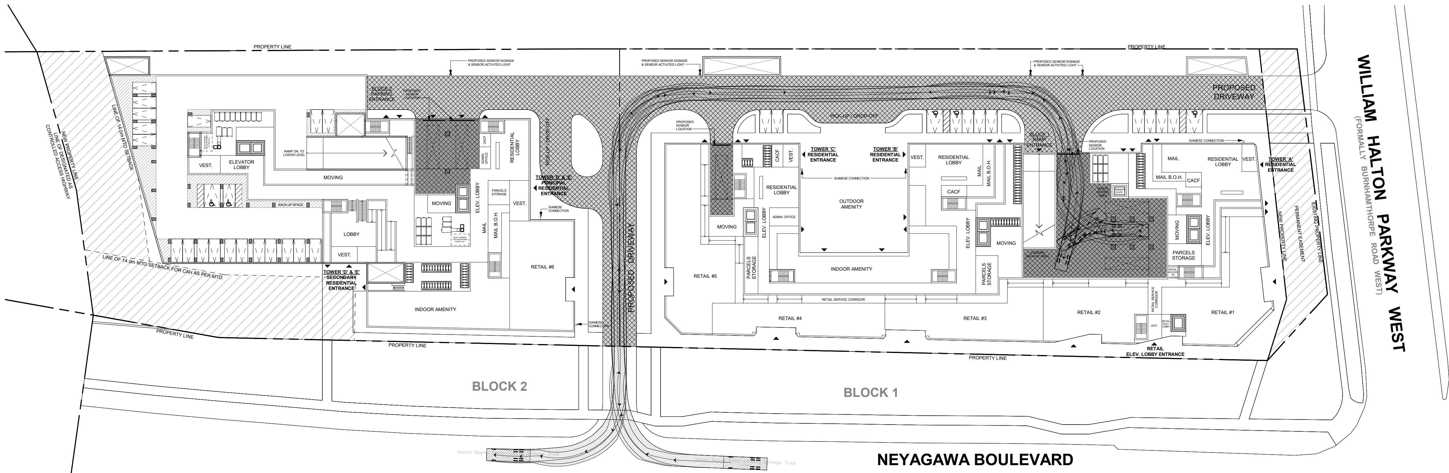
2 Waste Collection Vehicle Movement Diagram - Tower 'A' - Residential
