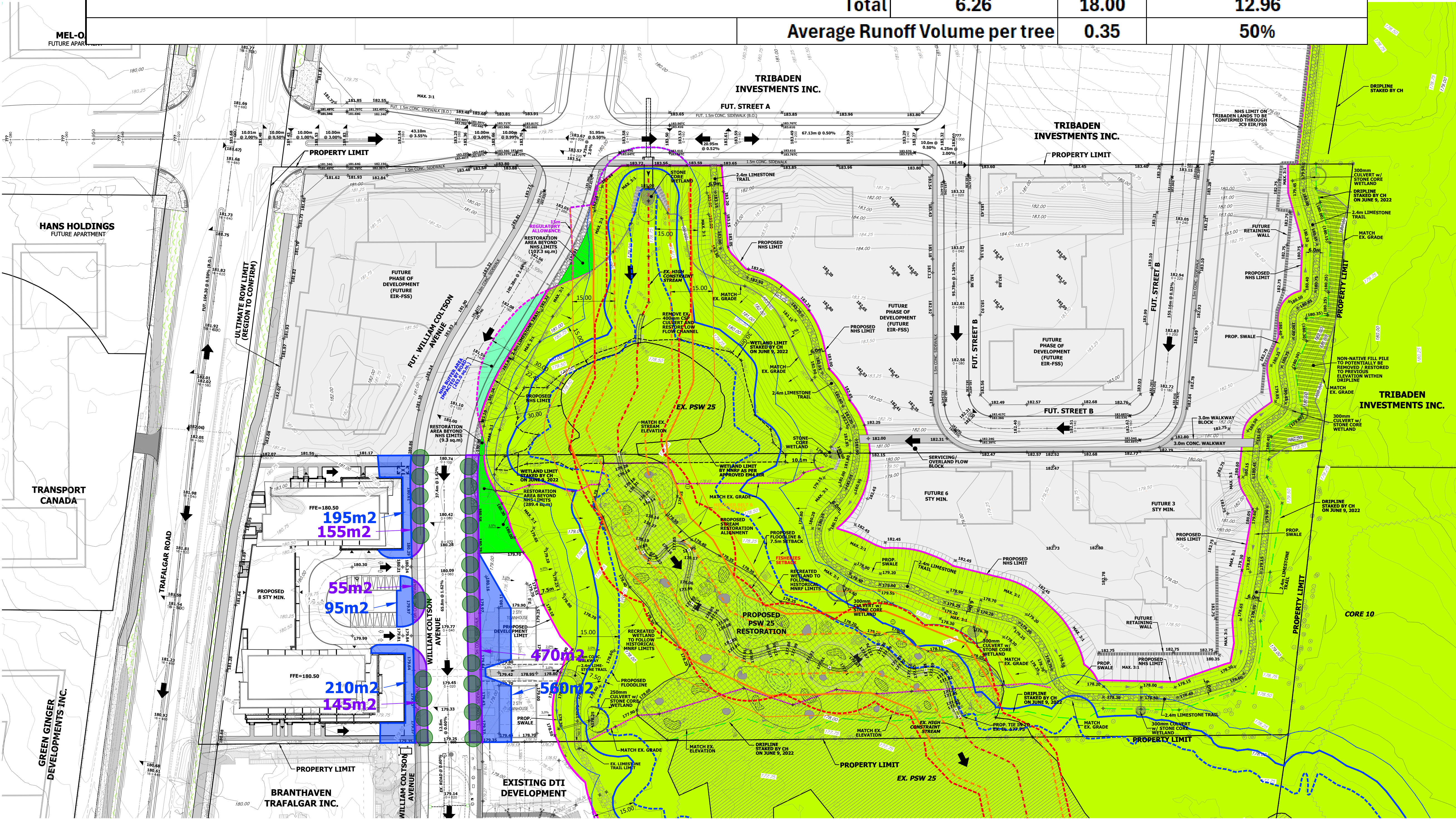
Figure A - Approximate Drainage Areas to tree pits
