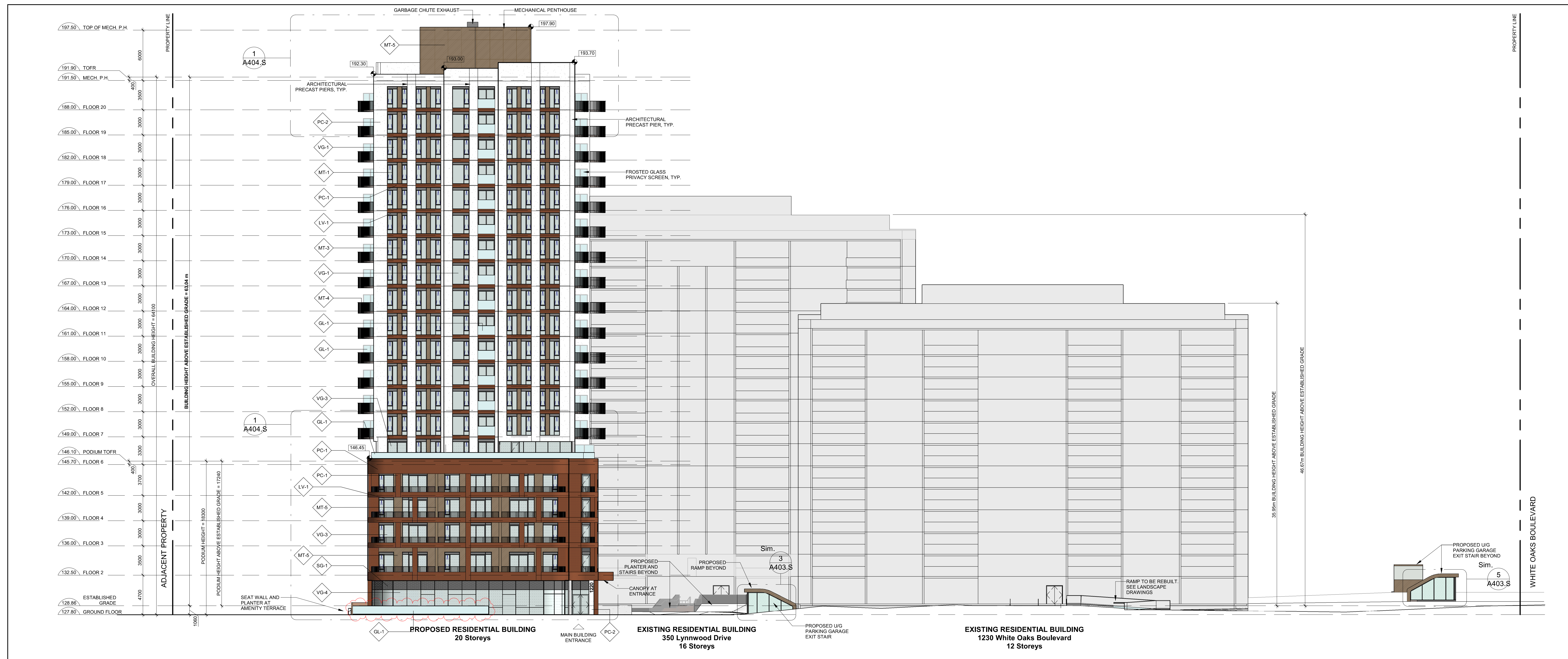
1 A401.S South Elevation
