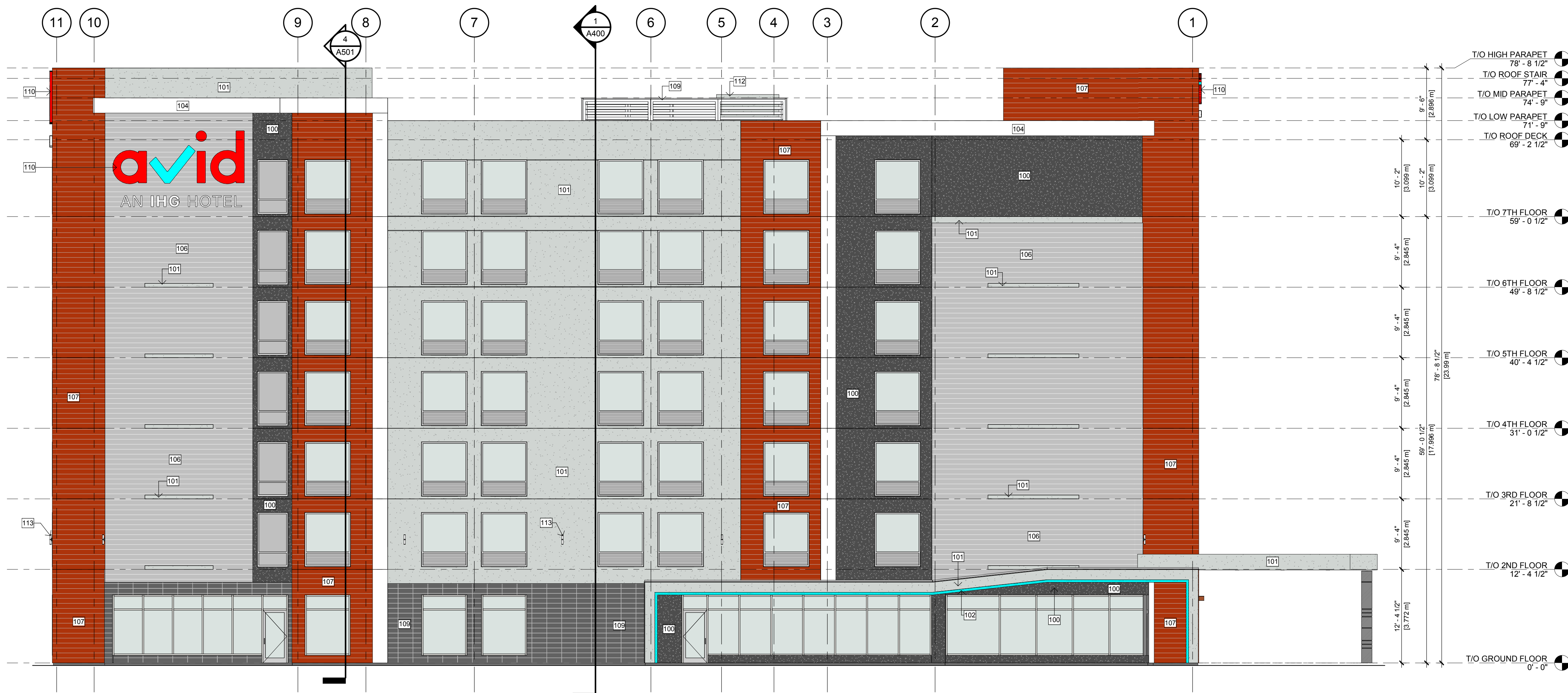
1 NORTH ELEVATION A301 1/8" = 1'-0"
