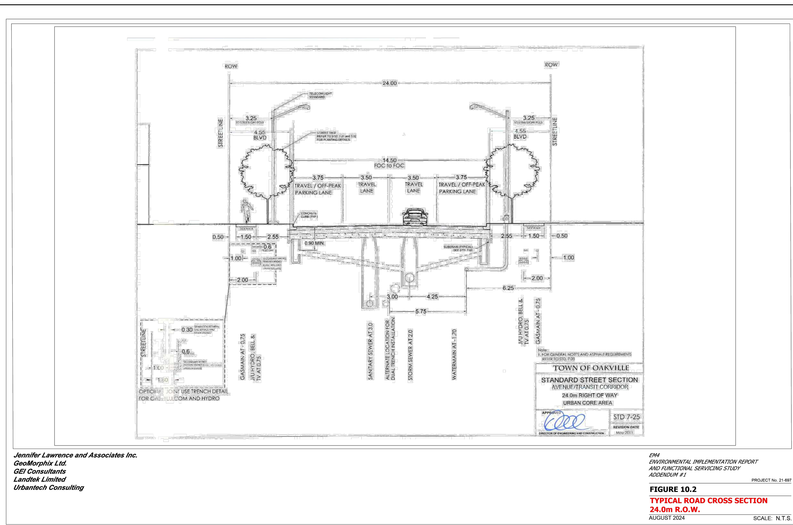
3 24m STREETSCAPE SECTION B-B'
