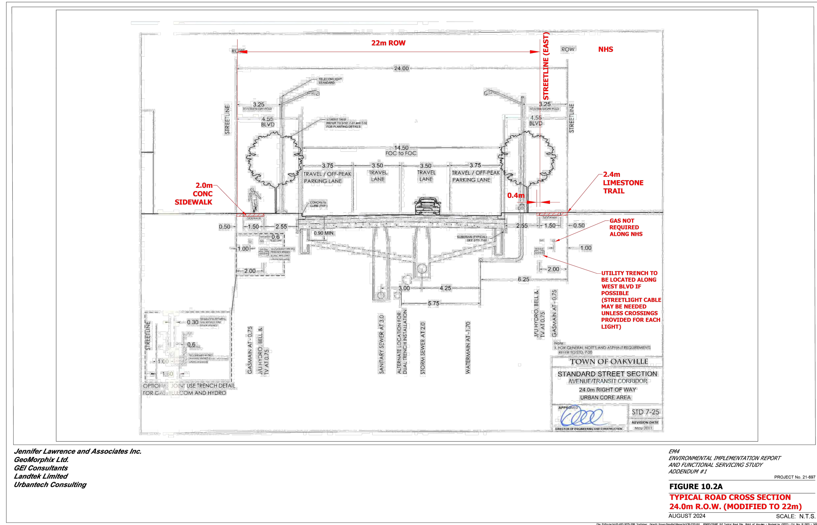
2 22m ROW STREETSCAPE SECTION A-A'
