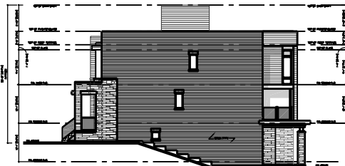
RIGHT SIDE ELEVATION 'A' DUAL-FRONTAGE TOWNS BLOCK 2
