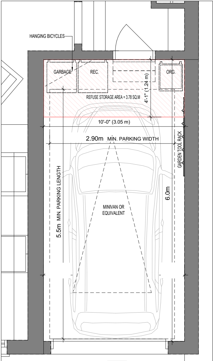
TYPICAL SINGLE CAR GARAGE SIZE (REAR ENTRY)
