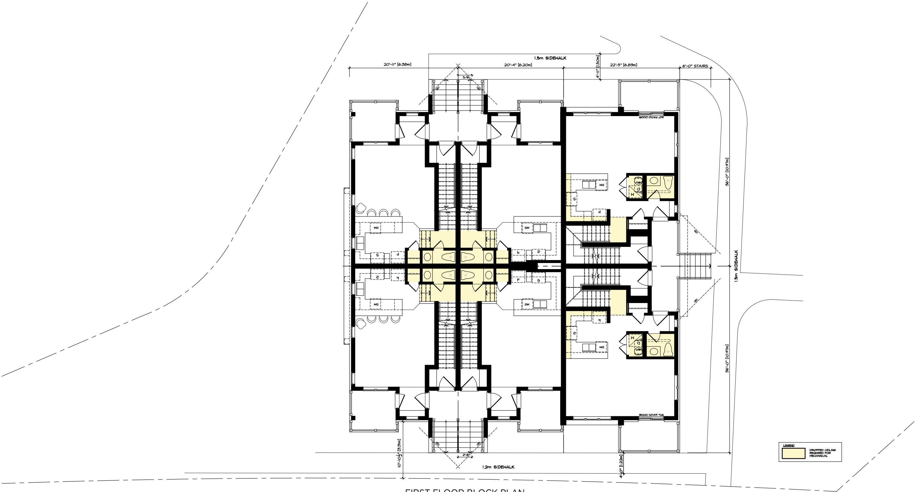
FIRST FLOOR BLOCK PLAN ELEVATION B
