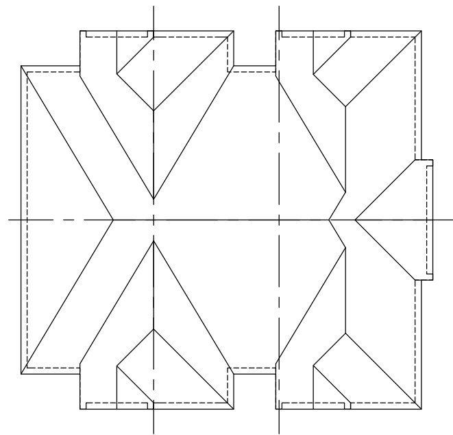
ROOF PLAN ELEVATION 'B'
