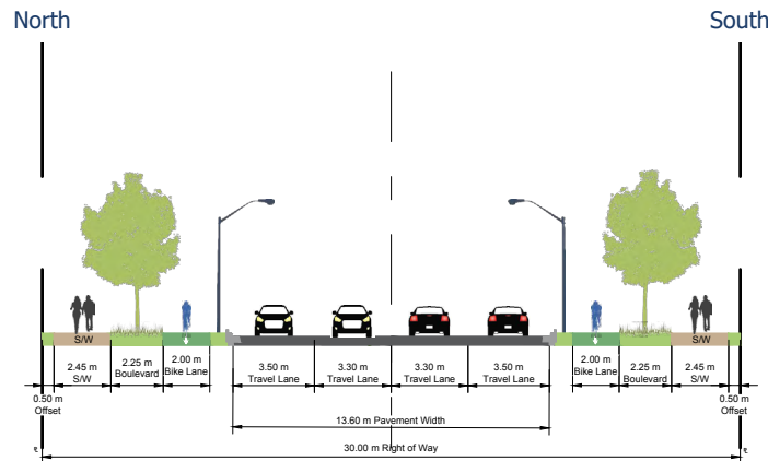
Cross-section - Prepared by BA GROUP
