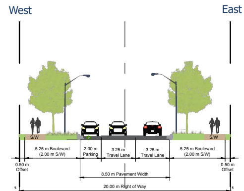
Cross-section - Prepared by BA GROUP
