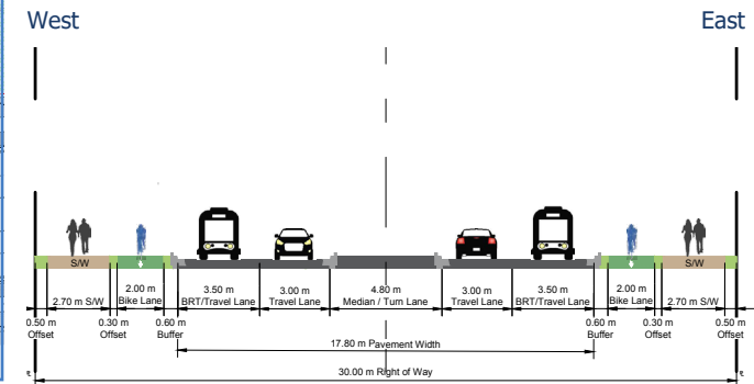
Cross-section - Prepared by BA GROUP
