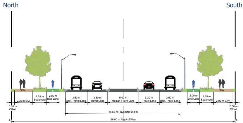
Cross-section - Prepared by BA GROUP
