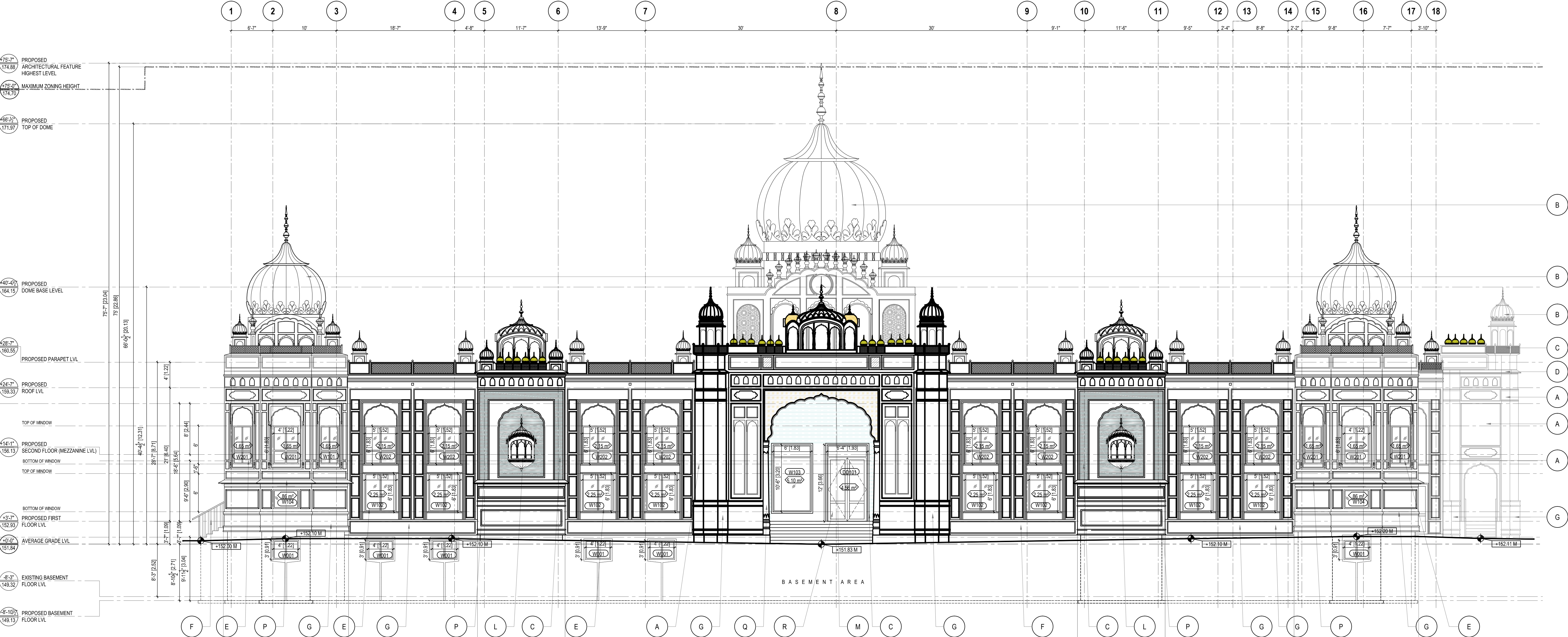
1 LEFT SIDE ELEVATION ( FACING PINE GLEN ROAD)
