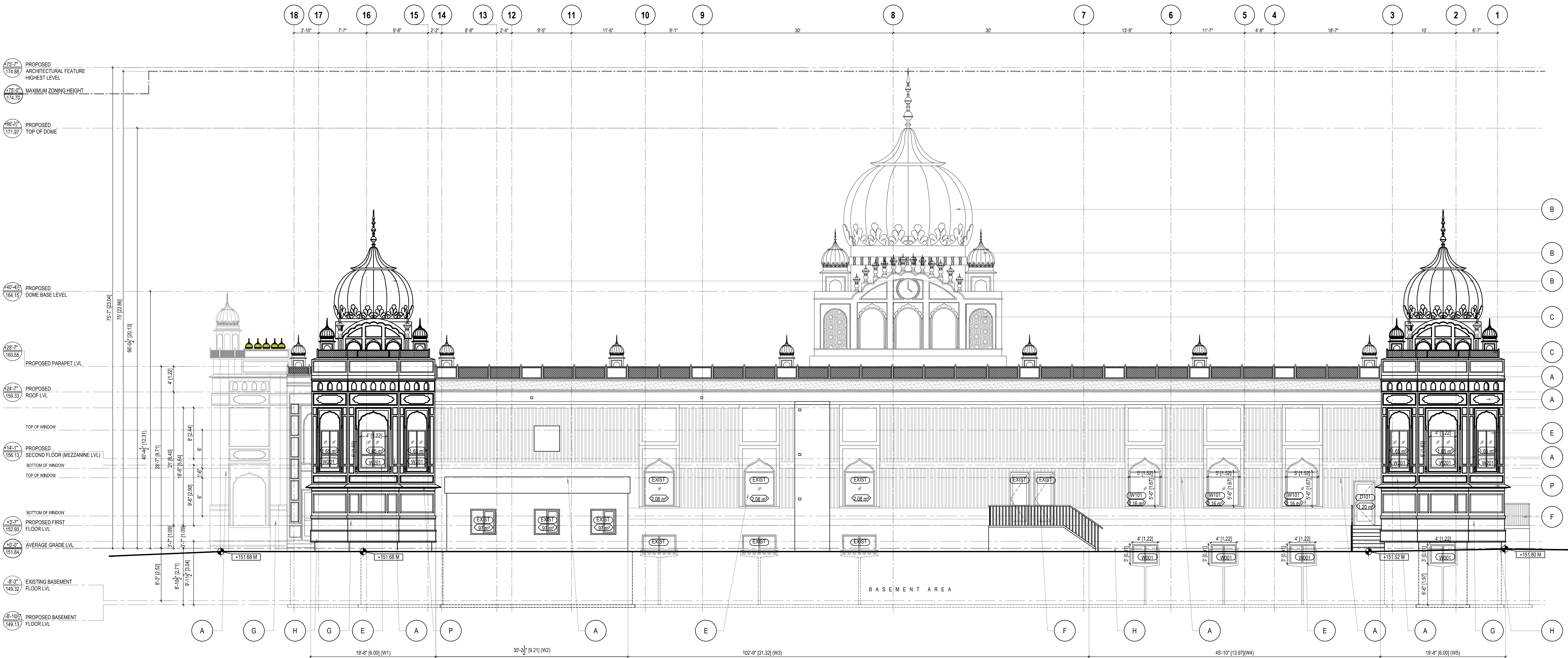
1 RIGHT SIDE ELEVATION (FROM WEST OAK TRAIL)
