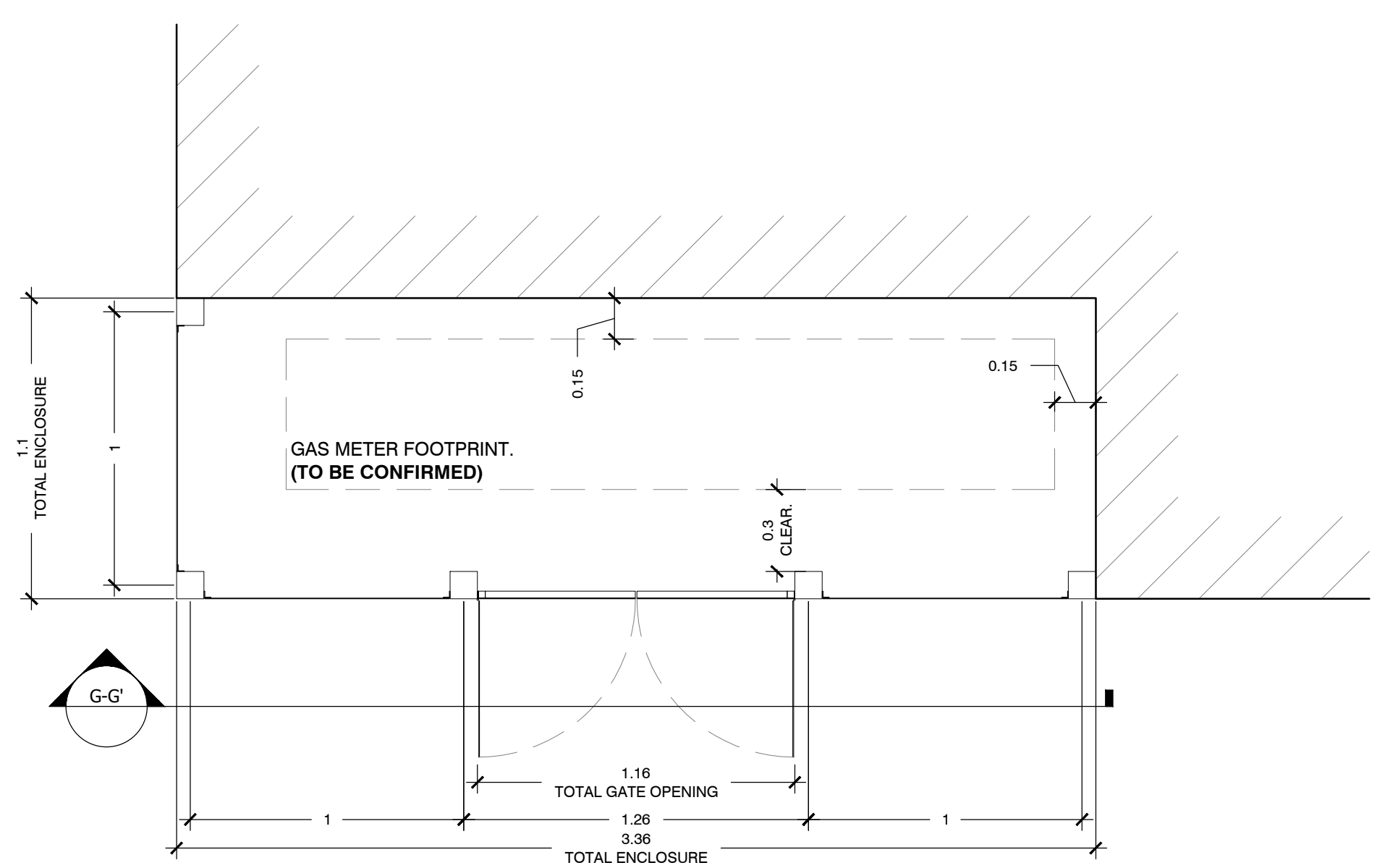
GAS METER SCREEN PLAN
