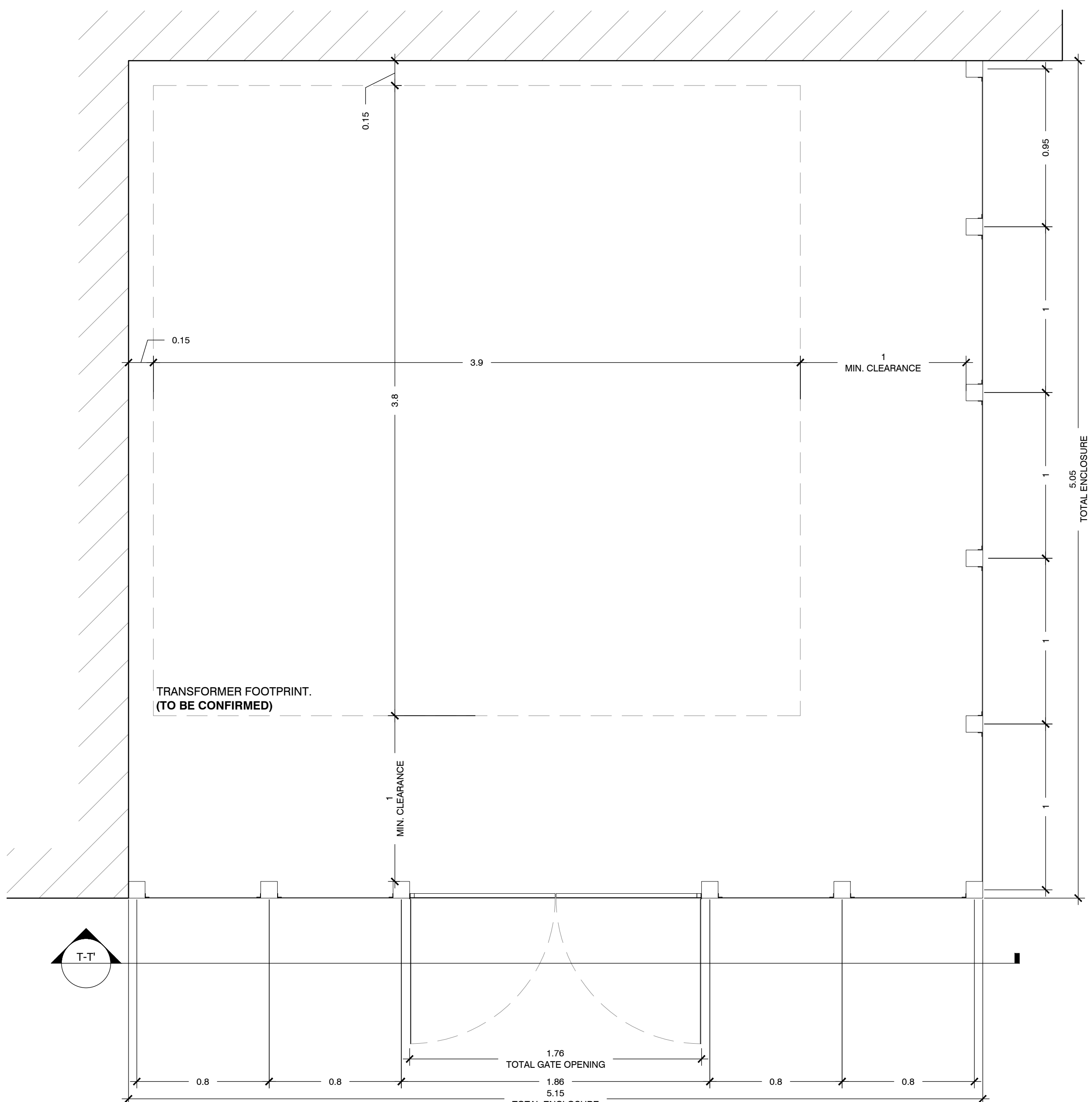
TRANSFORMER SCREEN PLAN
