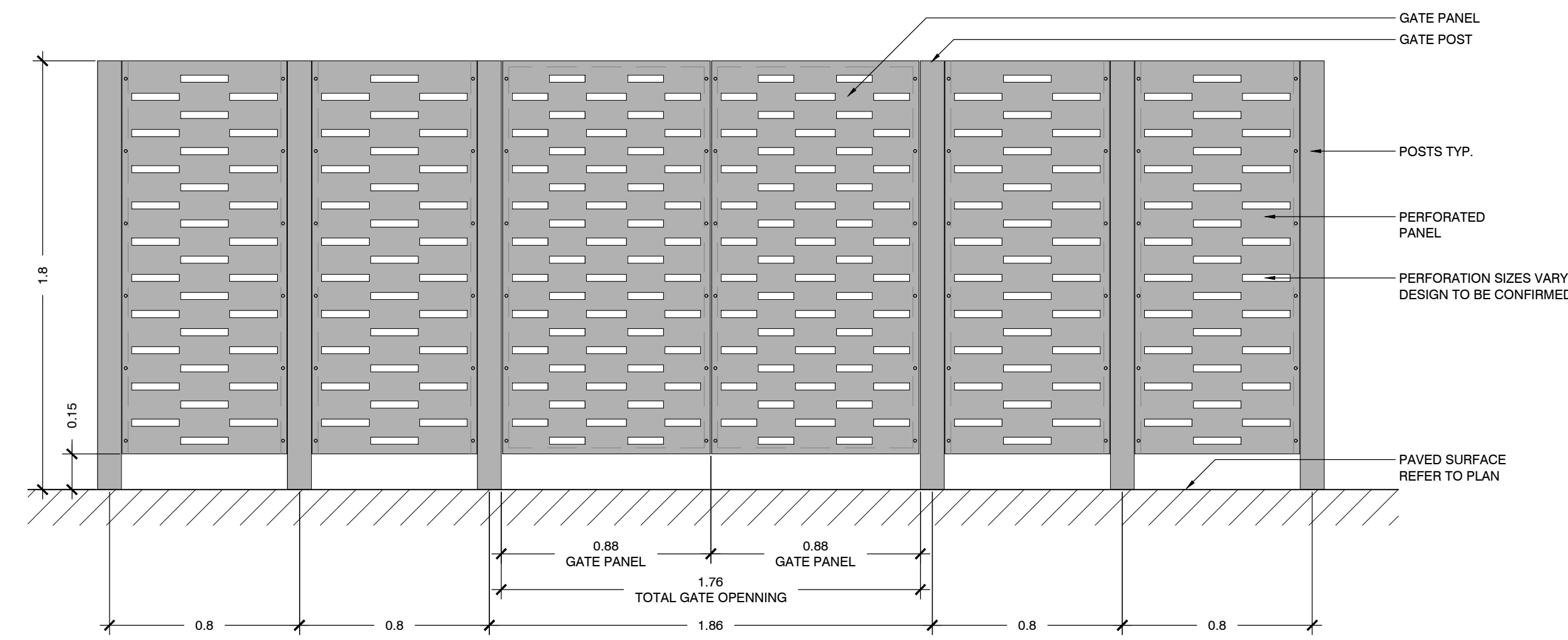
TRANSFORMER SCREEN ELEVATION T-T'
