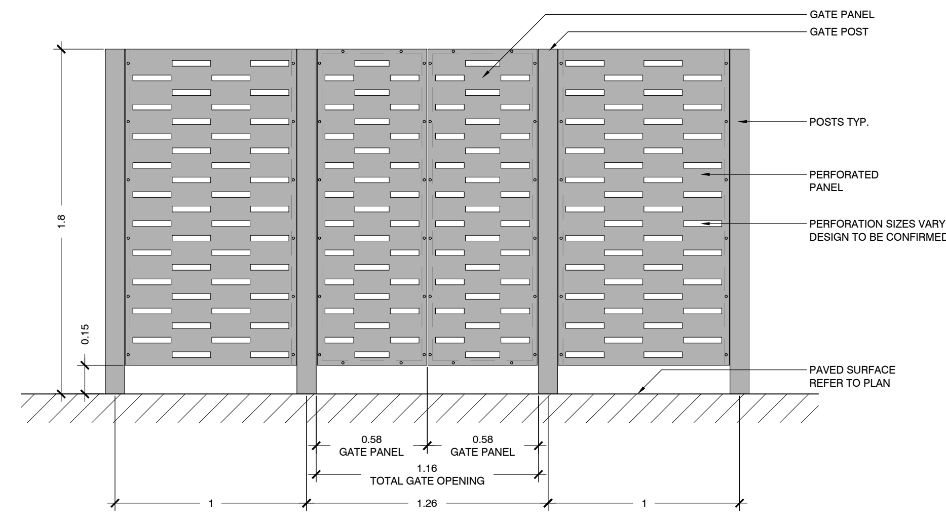
GAS METER SCREEN ELEVATION G-G'
