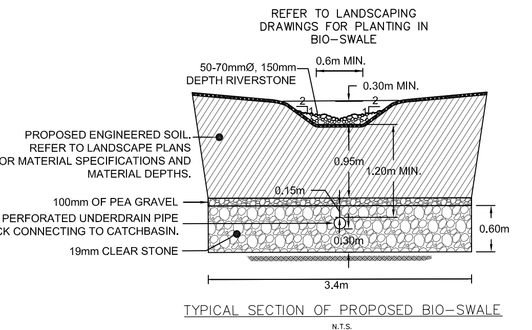
TYPICAL SECTION OF PROPOSED BIO-SWALE N.T.S.
